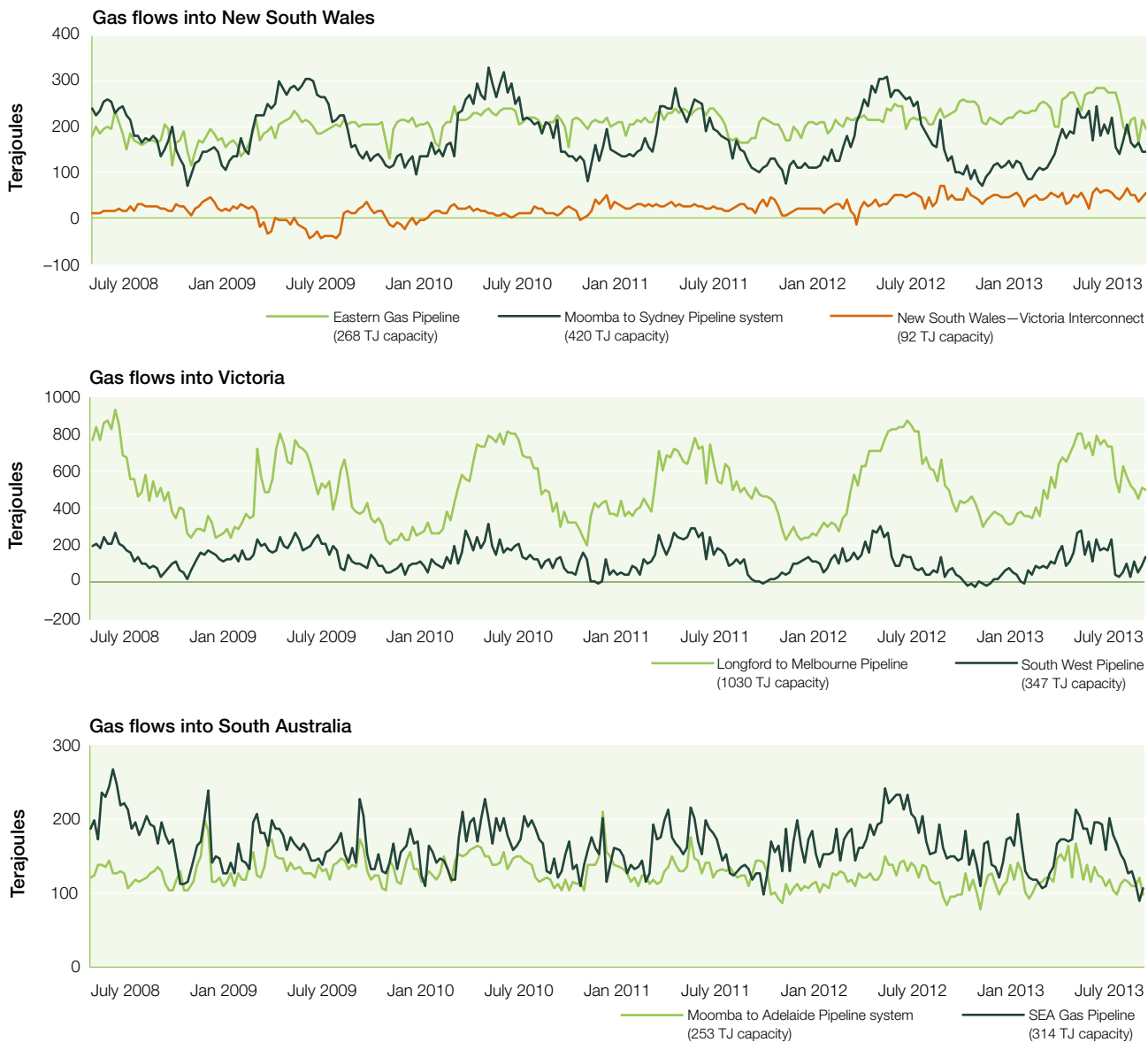
Figure 3.9 Gas flows in eastern Australia
