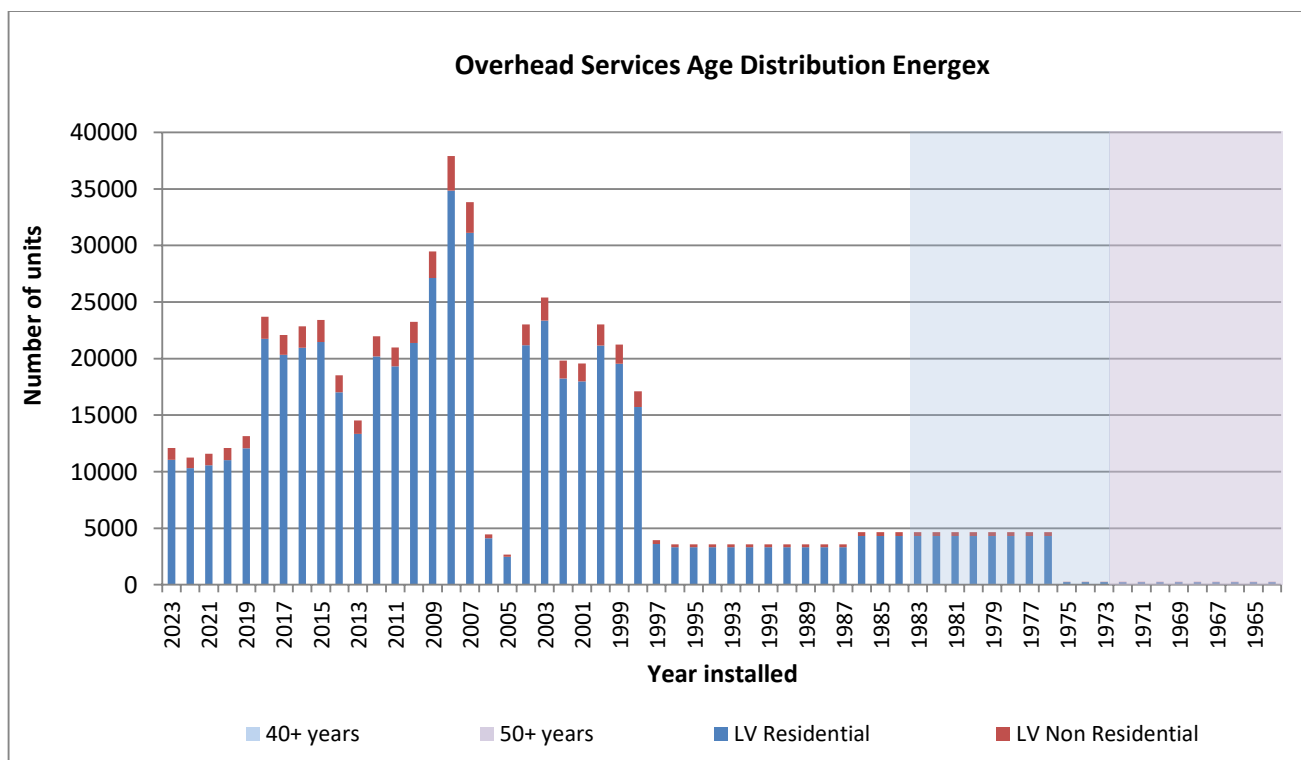
Figure 5: Age Profile Overhead Services - Energex
