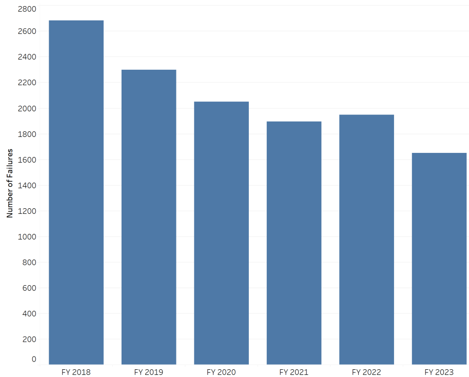
Figure 15: Overhead Service Failure Quantity – Energex
