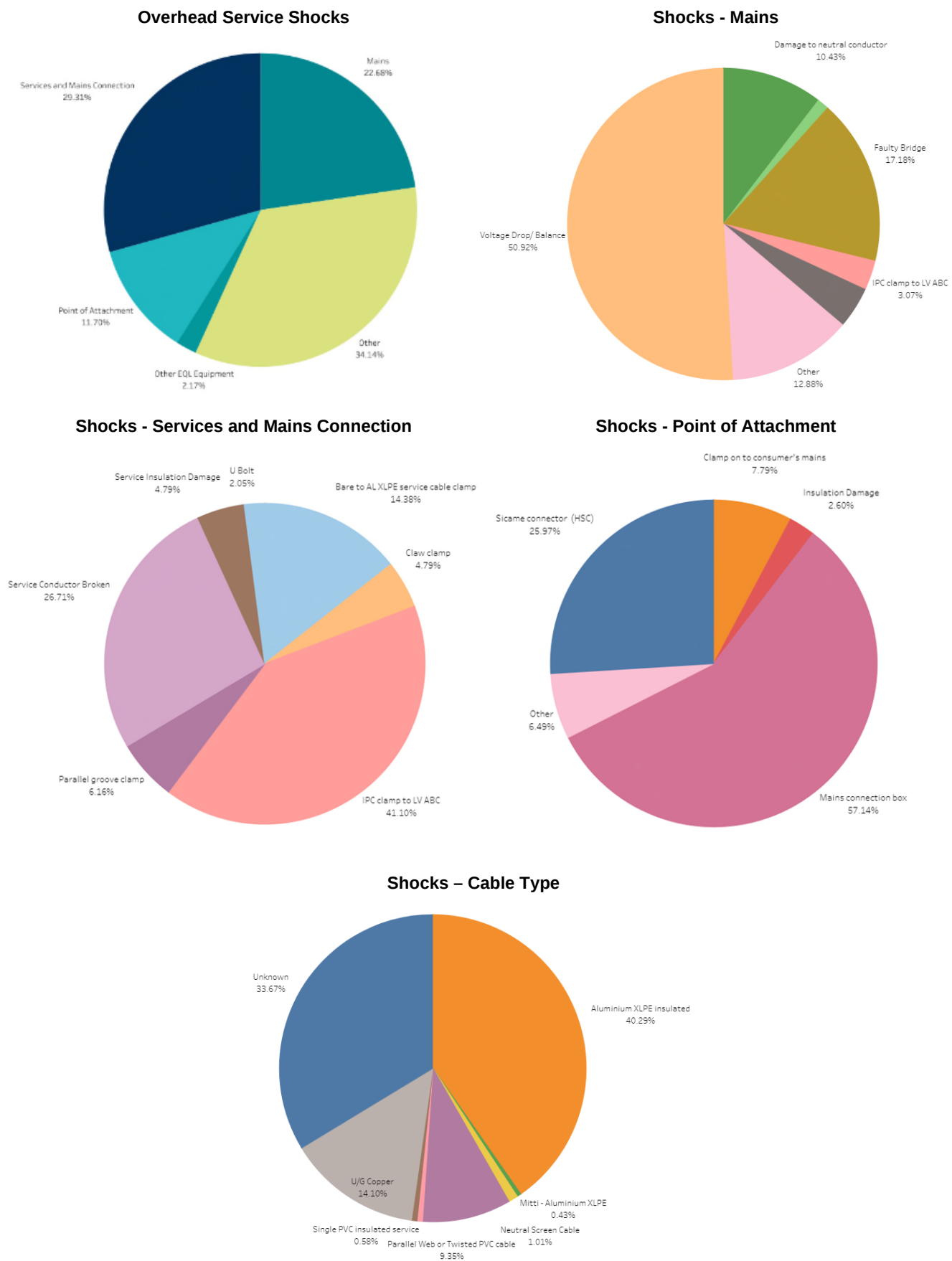
Figure 13: Average (6 Years) Overhead Service Shock Rate – Energex
