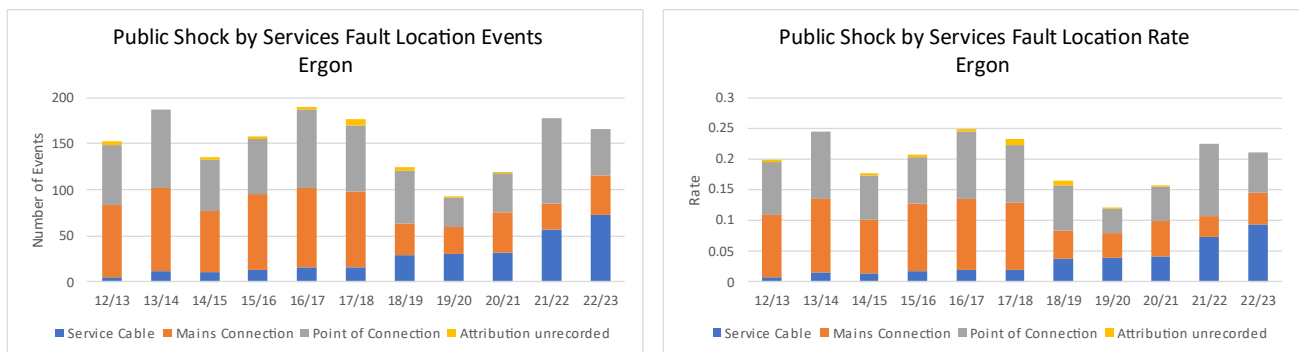
Figure 7: Overhead Service Related Shock Performance – Ergon Energy
