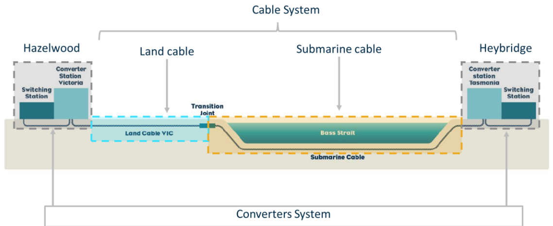
Figure 7: Stage 1 cable system and converters system
