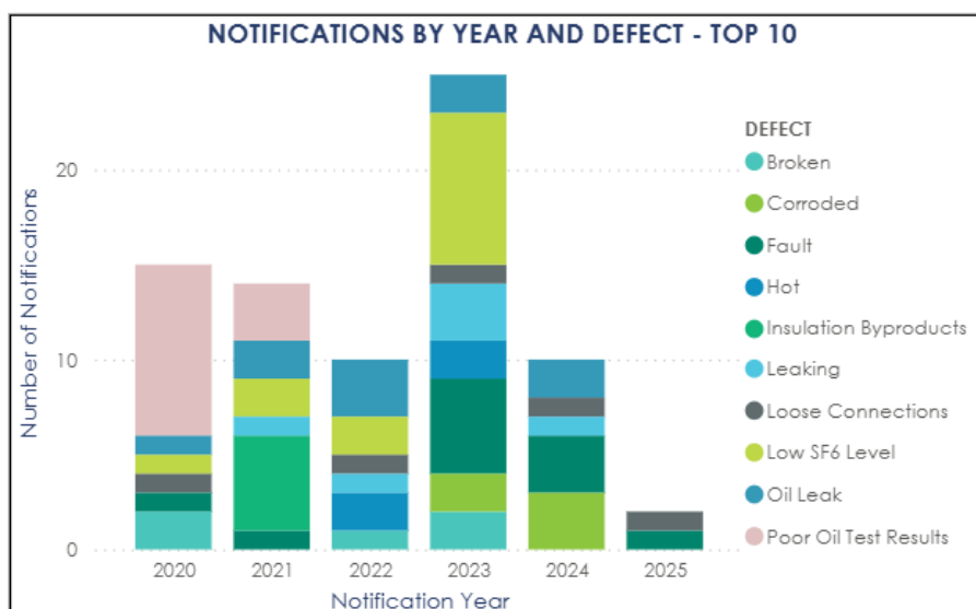
Figure 13: ZA and ZK Notifications vs Defect 2020 – mid 2025 (top 10)
