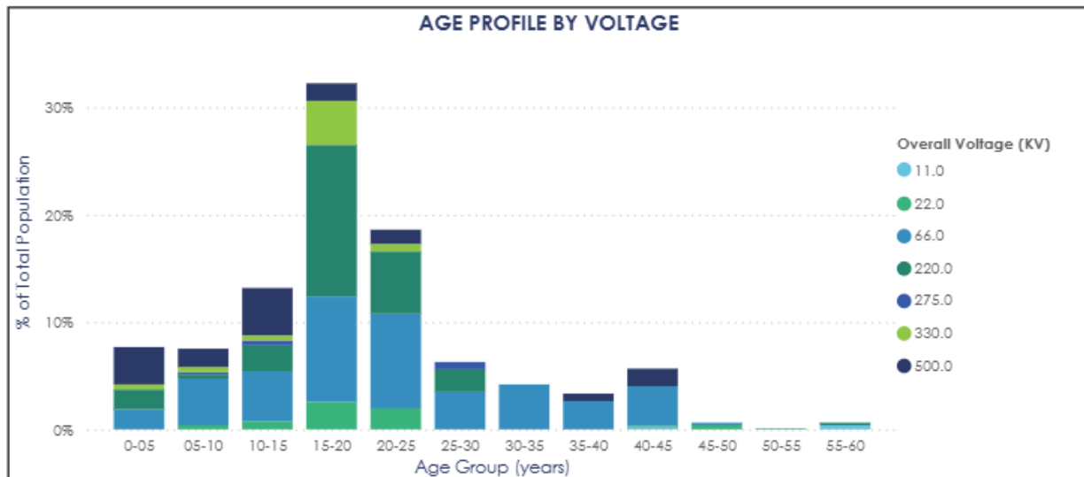
Figure 7: Current Transformer Age by Service Voltage
