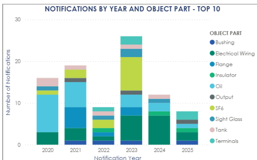
Figure 14: ZA and ZK Notifications vs Object Part affected 2020 – mid 2025 (top 10)
