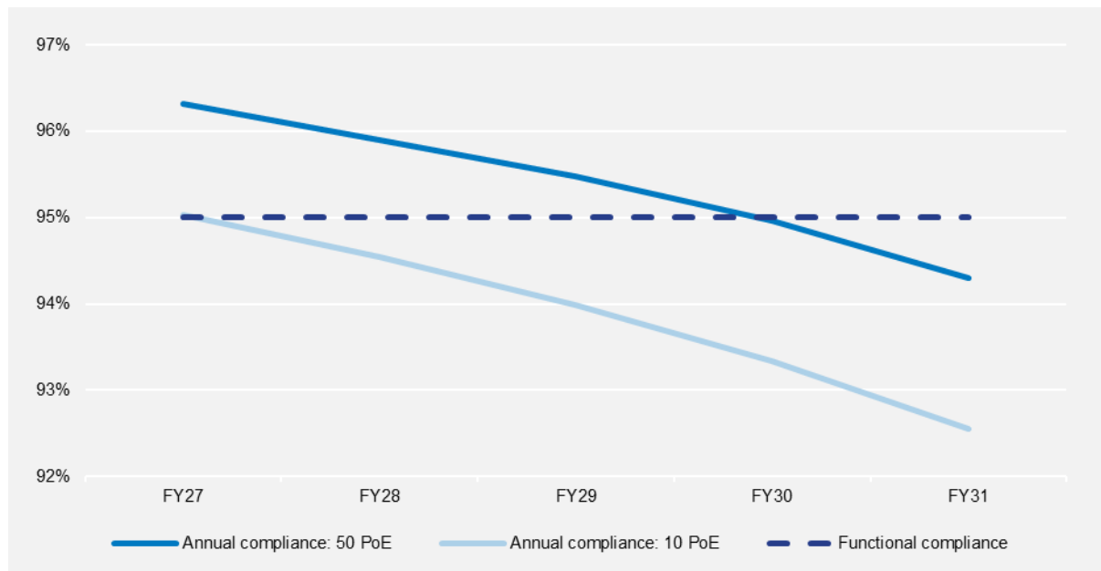
FIGURE 6 VOLTAGE COMPLIANCE FORECAST
