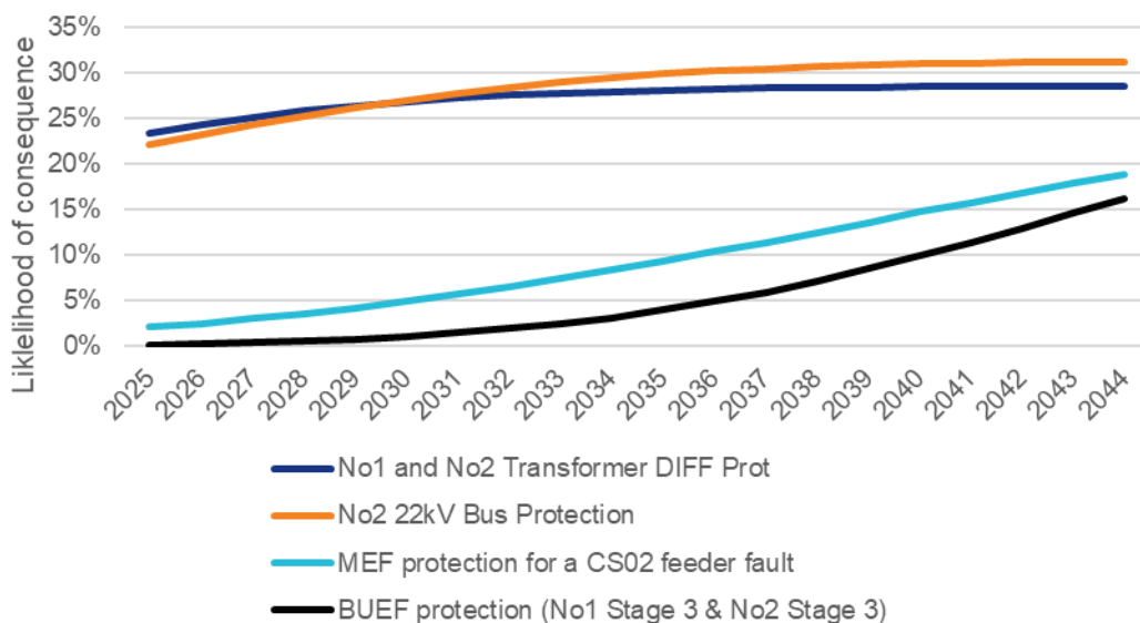
Figure 4-3 Secondary equipment likelihood of consequence based on Weibull distribution
