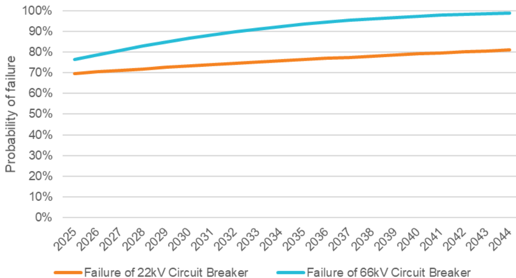
Figure 4-2 Primary equipment probability of failure based on Weibull distribution
