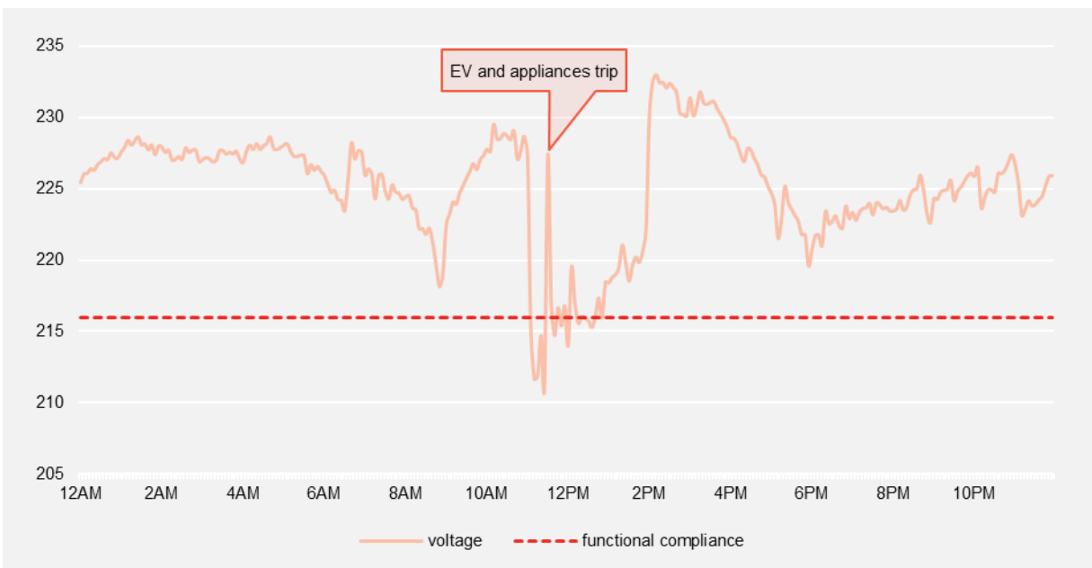
FIGURE 12 DAILY OVO CUSTOMER VOLTAGE (VOLTAGE)
