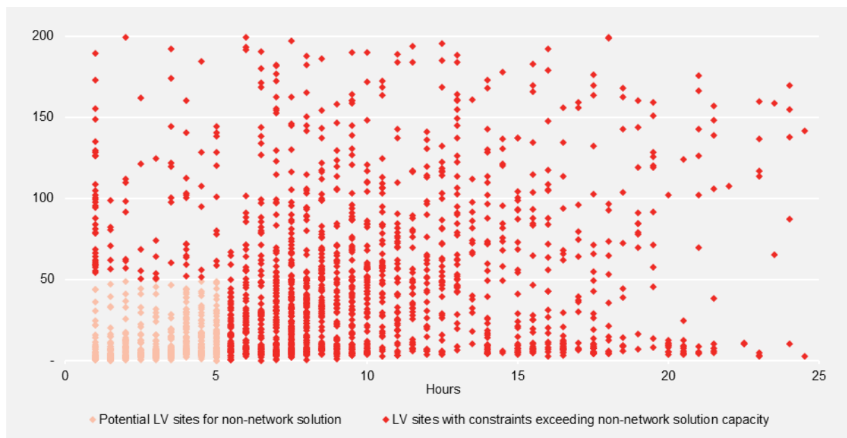
FIGURE 9 SUITABILITY OF NON-NETWORK SOLUTIONS (KW)
