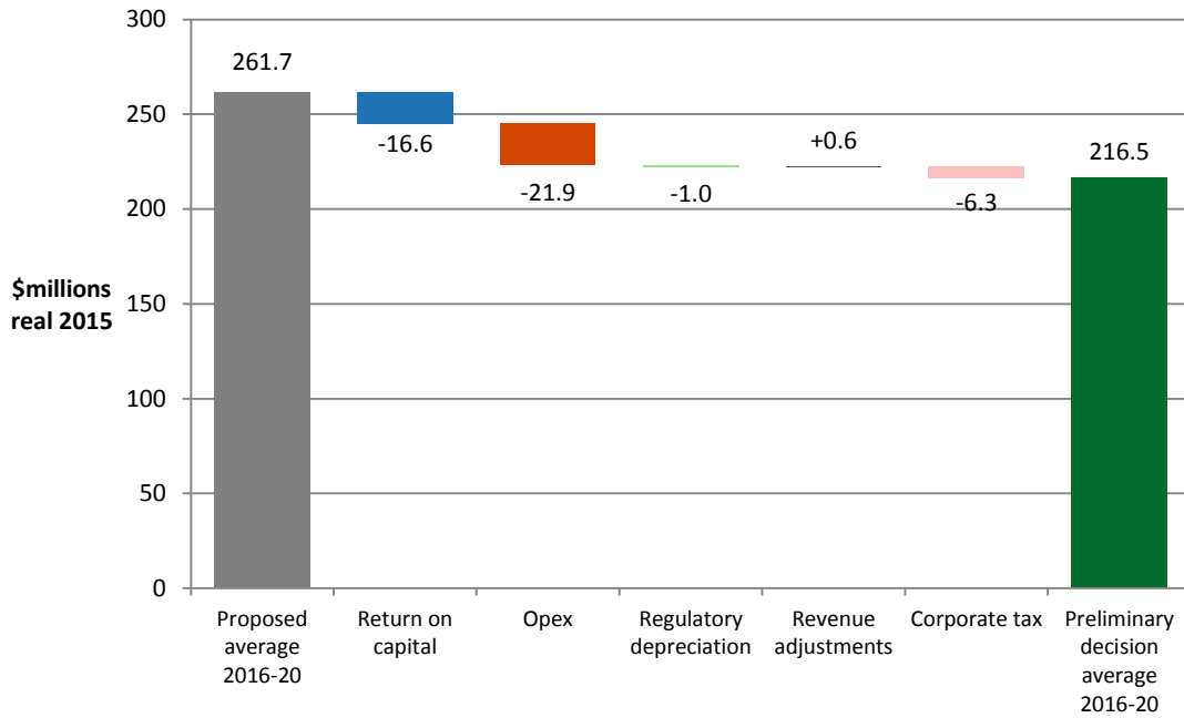
Figure 2 AER's preliminary decision and Jemena's proposed annual building block costs ($ million, 2015)
