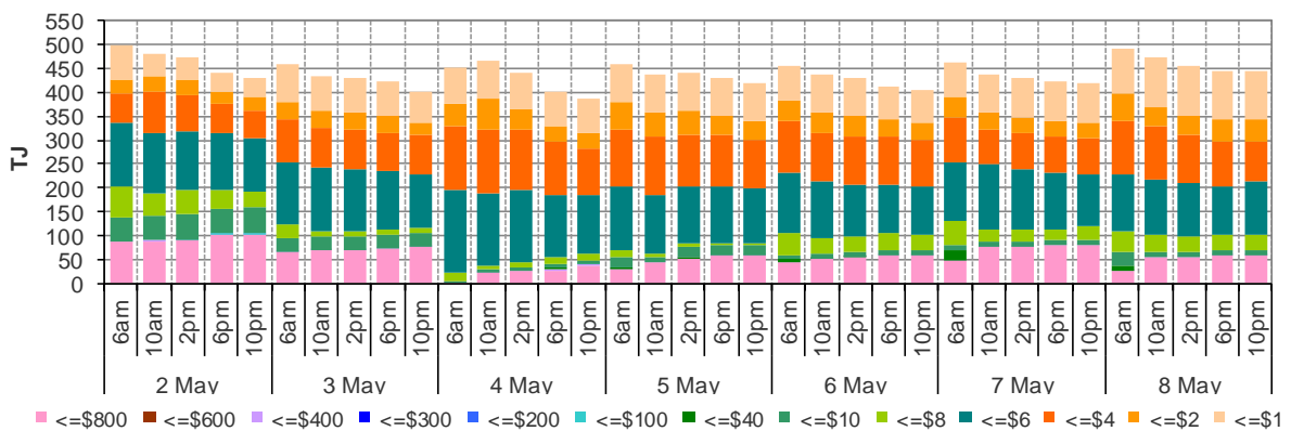
Figure 1.5: Metered Injections by System Injection Point (TJ) 8
