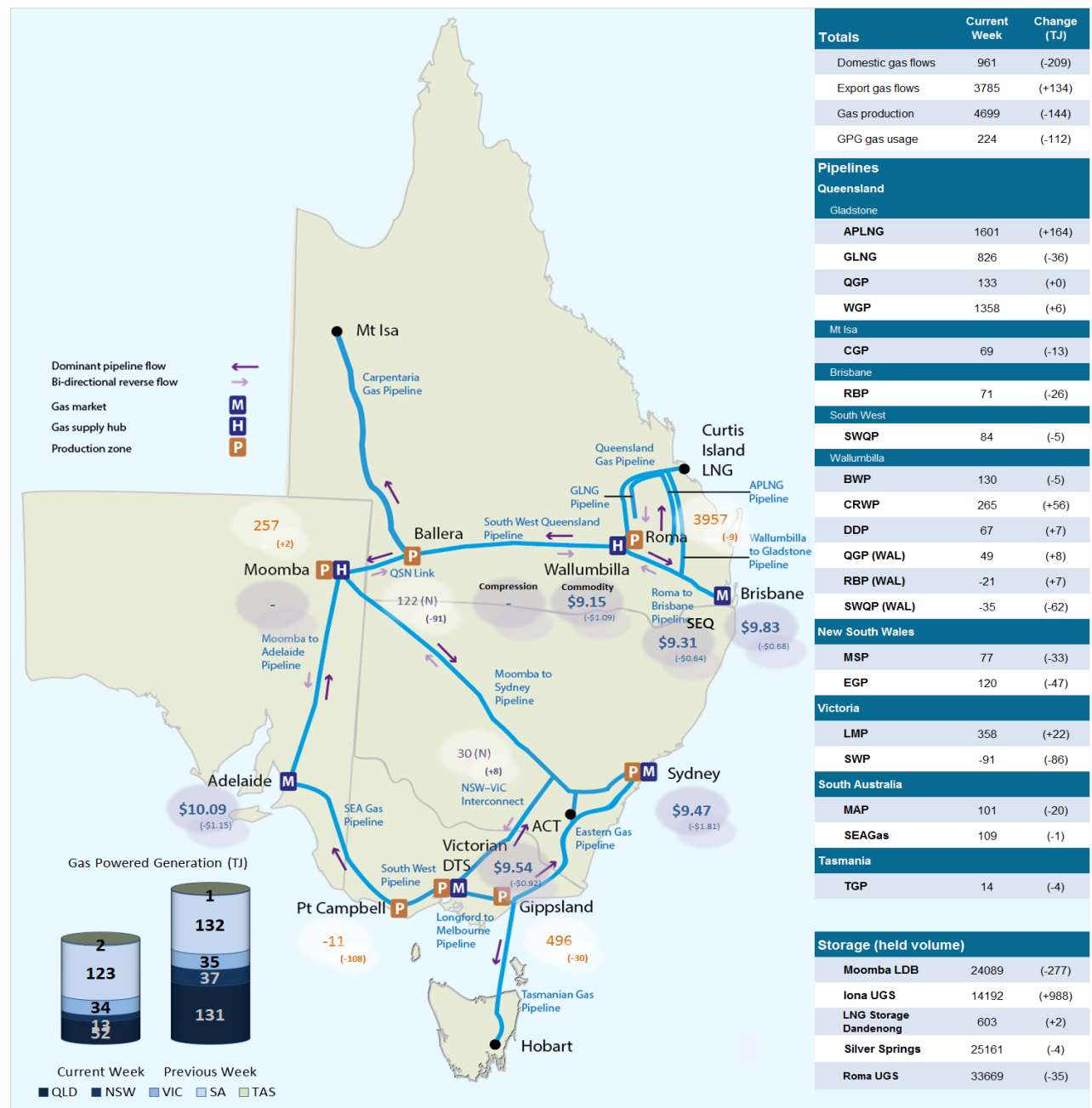
Figure 5.1: Gas market data ($/GJ, TJ); Bulletin Board flows (TJ) 13
