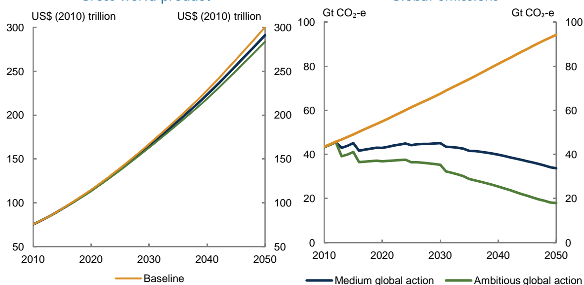
Chart 3.6: Global emissions and gross world product Gross world product Global emissions
