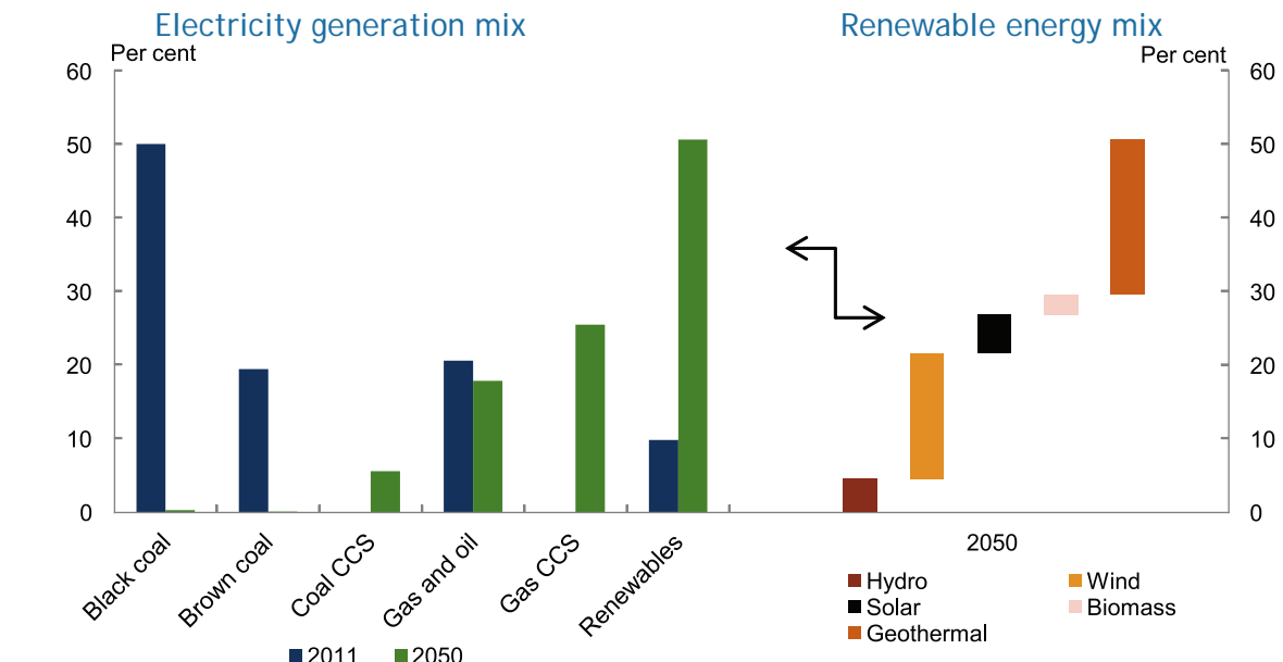
Chart 5: Electricity generation mix, core policy scenario
