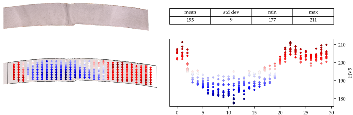
Figure 4 Cross seam weld of S1 and hardness HV5.
