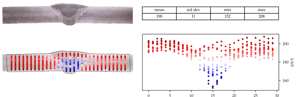
Figure 3 Cross girth weld of S1 and hardness HV5.
