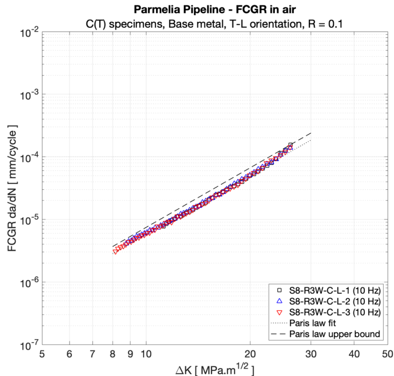
Figure 9 Fatigue crack growth rate for the transverse specimens of S8 sampled from BM.
