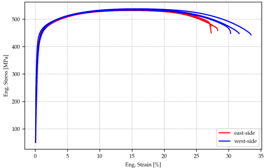
Figure 5 Engineering stress-strain curve from the base metal transverse specimens of section S1.
