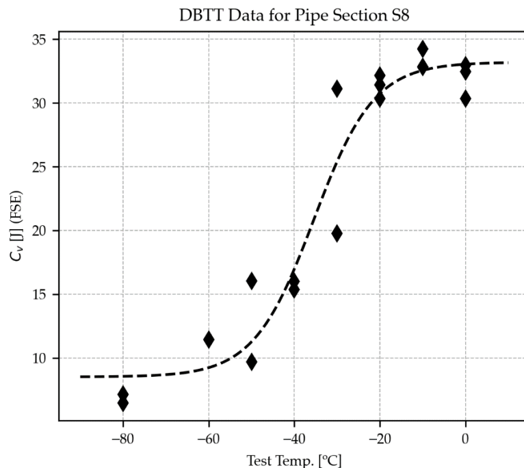
Figure 7: DBTT data for Charpy samples from the west-side of S8.
