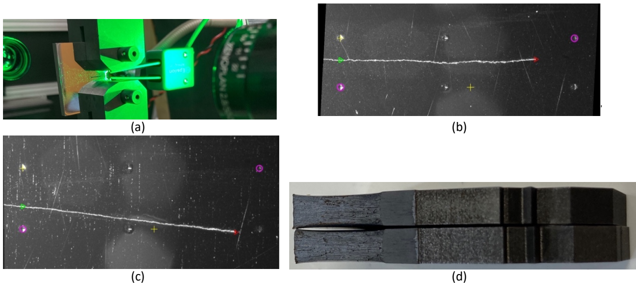
Figure 8 (a) Test setup on the tensile machine showing the C(T) specimen pinned on the clevises with the clip gauge and the two cameras used to monitor the crack during the pre-cracking phase. (b) Near straight and centered propagation of the fatigue crack in a girth weld centreline specimen from S8. (c) Deviation of crack path out of the symmetry plane in the heat-affected zone of a girth weld specimen from S8. (d) Illustration of the fracture surface after testing showing from left to right (i) the EDM notch, (ii) fatigue fracture from the fatigue pre-crack phase and (iii) ductile fracture from the toughness test.
