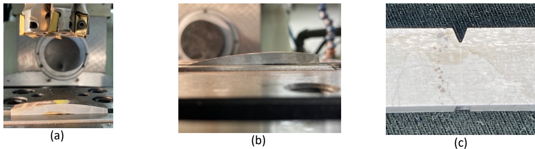
Figure 6 Preparation of Charpy specimens. (a) Milling of the top face, normal to the seam weld centreline. (b) The seam weld centreline was angled noticeably from the pipe's radial direction in several cases. (c) Notch after etching of the specimen's surface. The seam weld centreline is visible in the picture.
