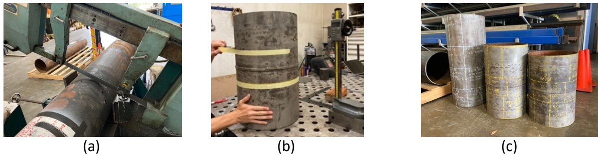
Figure 1 Preparation of the sections for sampling. (a) Ring cut out of S8 using a band saw. (b) Marking and measuring of the rings to locate the plates to be cut by water-jetting. (c) Completed marking from S1, S5 and S8.
