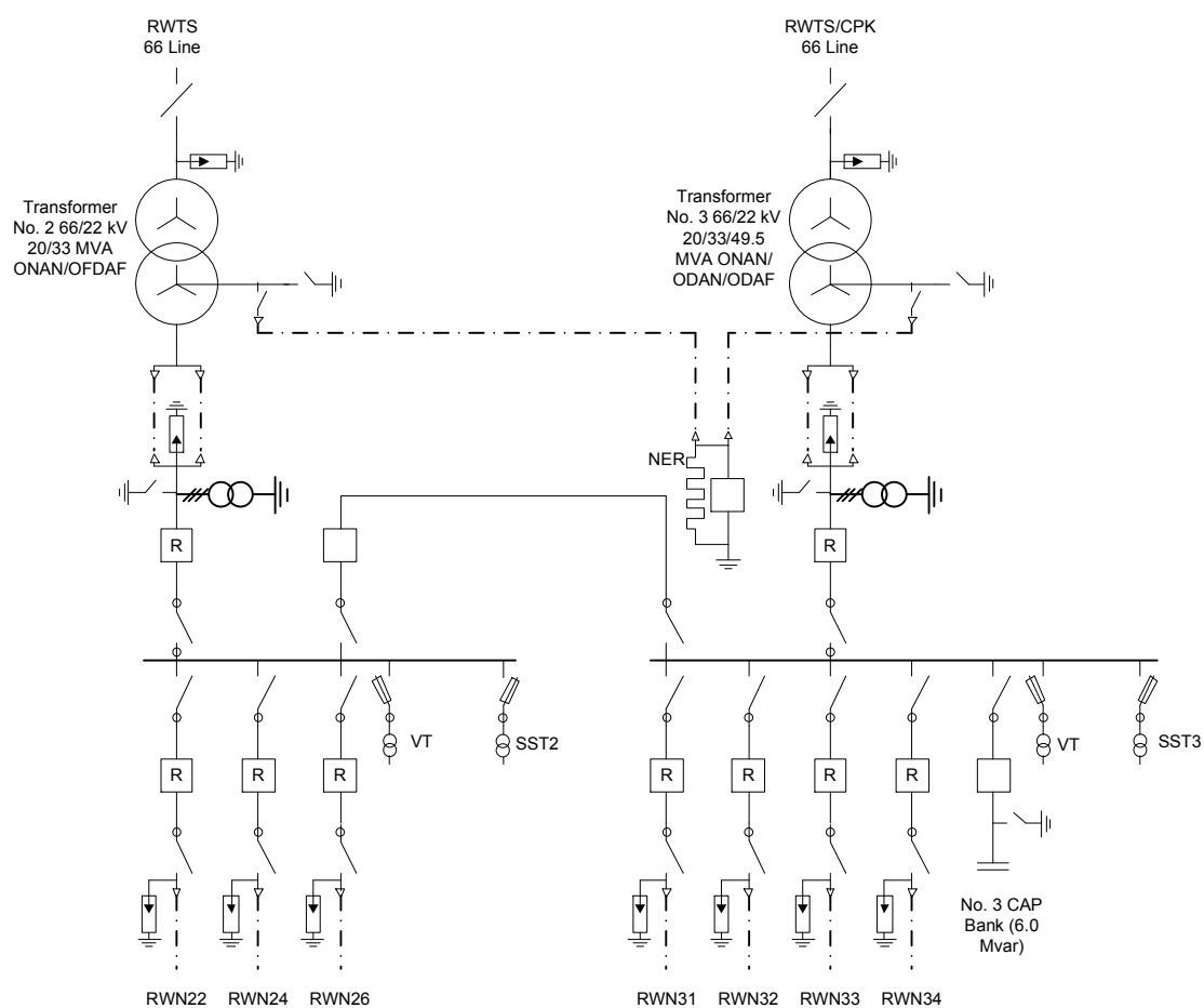
Figure 2: RWN Current Single Line Diagram
