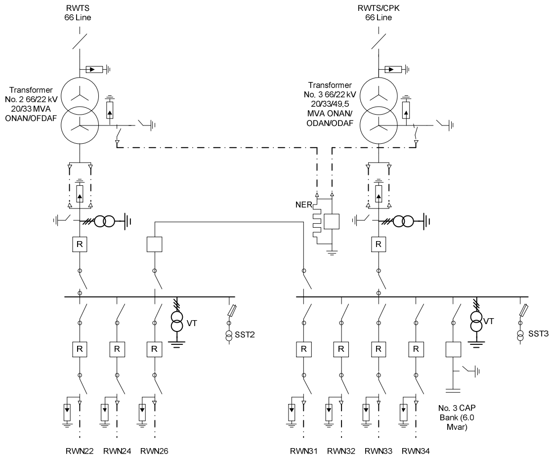
Figure 3: RWN proposed single line diagram
