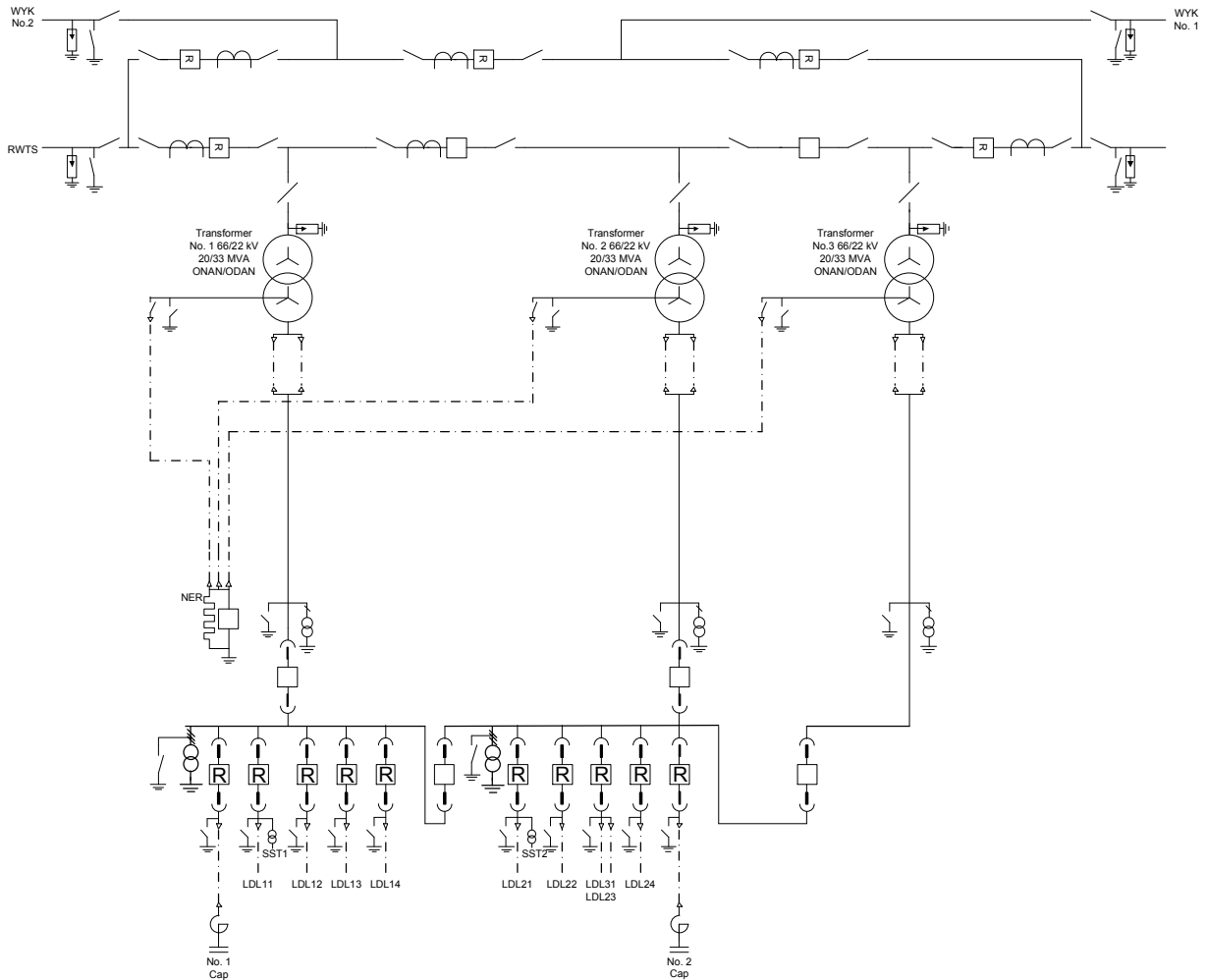
Figure 2: LDL Current Single Line Diagram
