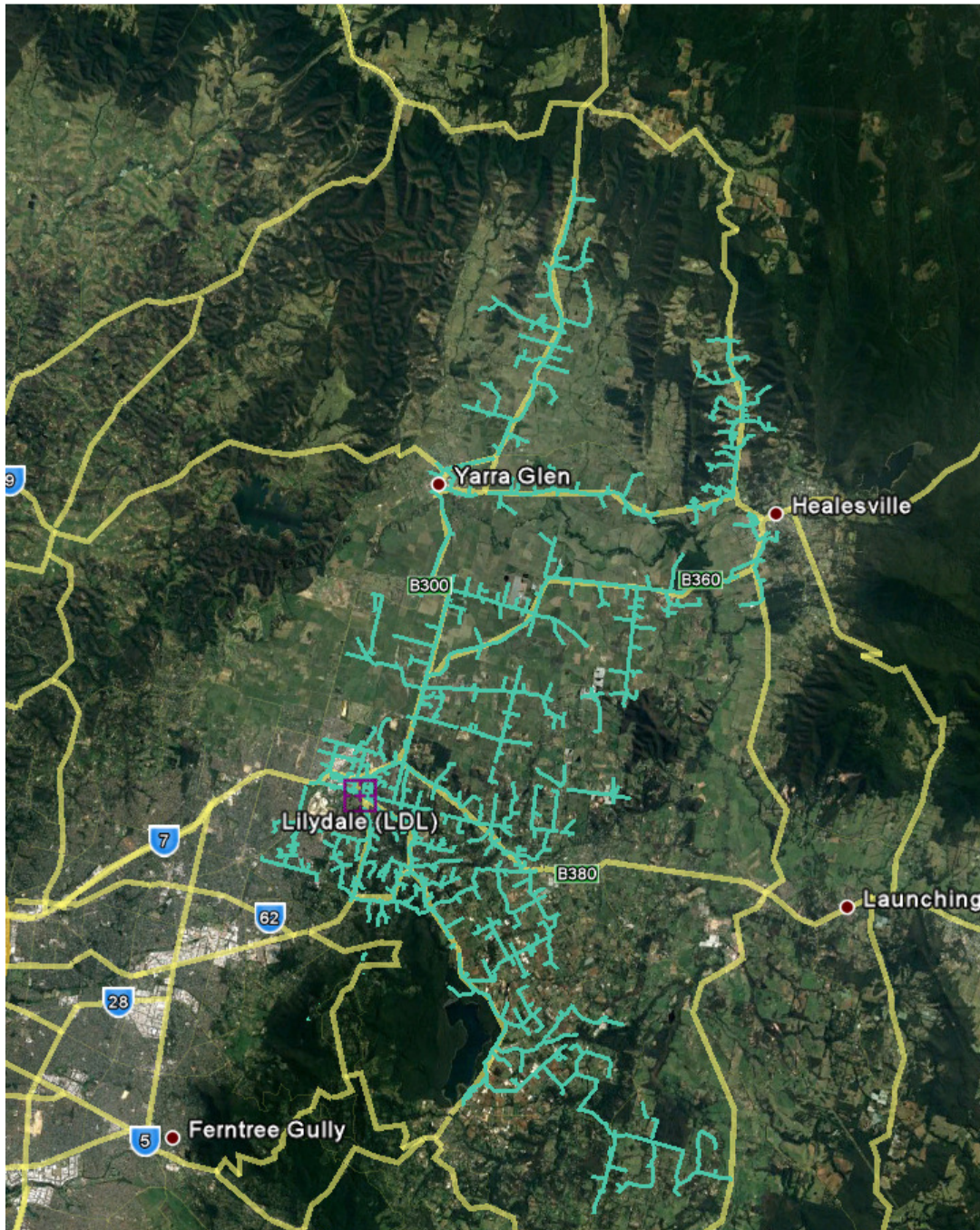
Figure 2: LDL 22kV feeders shown in blue
