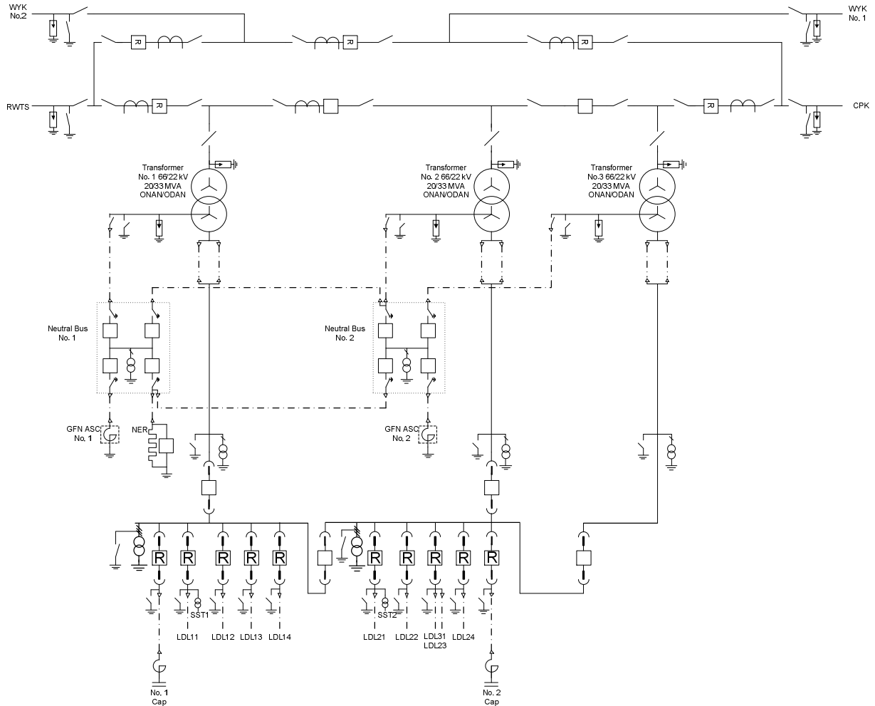
Figure 3: LDL proposed single line diagram
