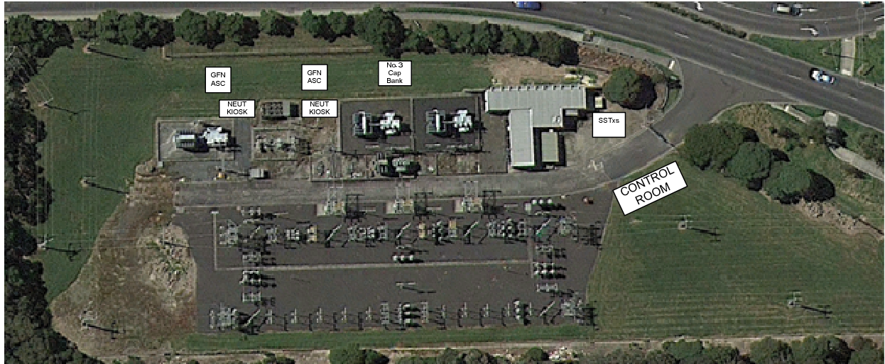
Figure 5: Aerial view of the LDL ZSS
