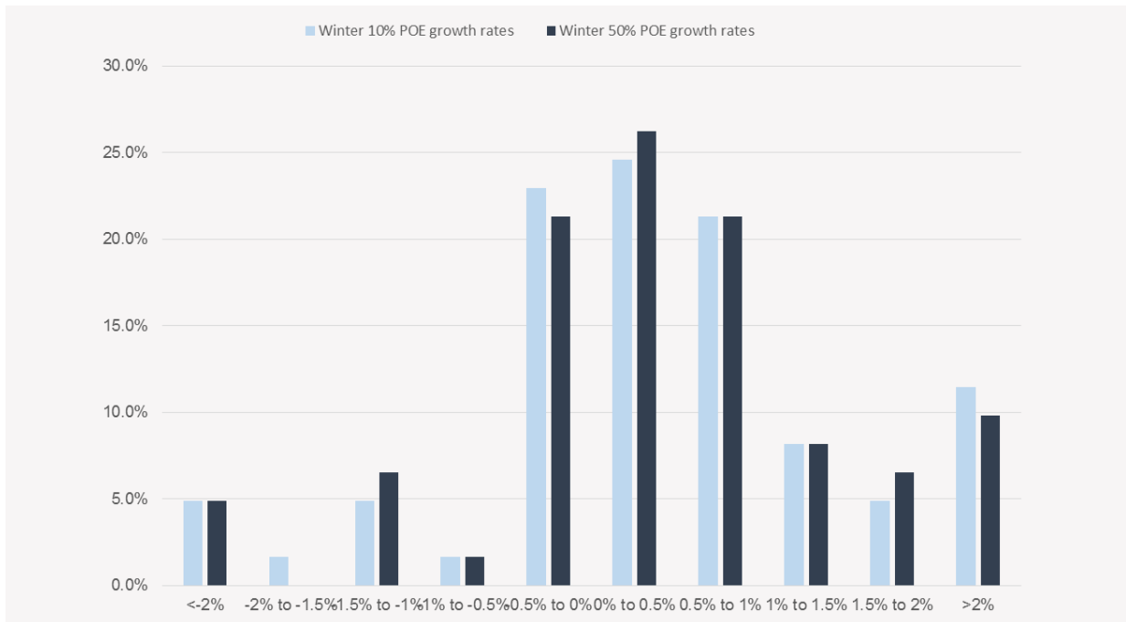
Figure 5 Distribution of winter MD growth rates for Victoria, 2014–23
