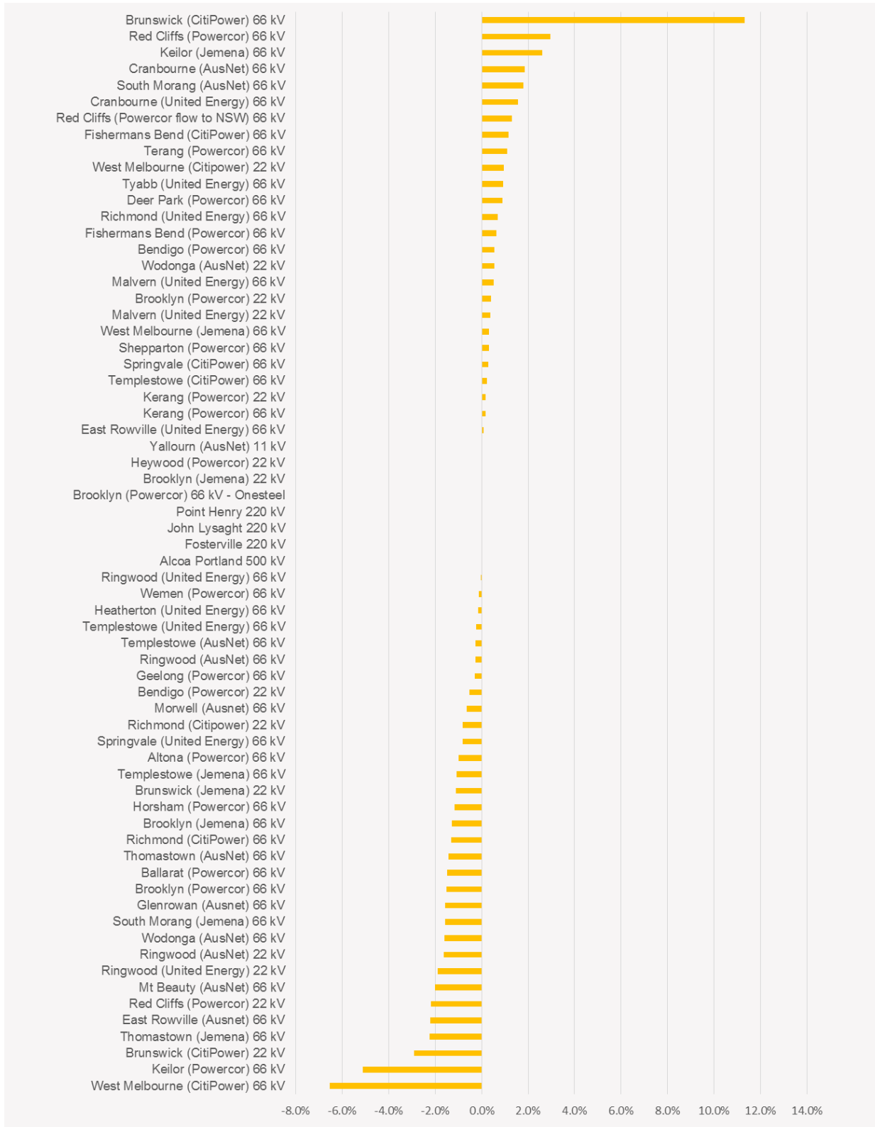
Figure 6 Victoria 10% POE summer 10-year average annual growth rates, 2014–15 to 2023–24
