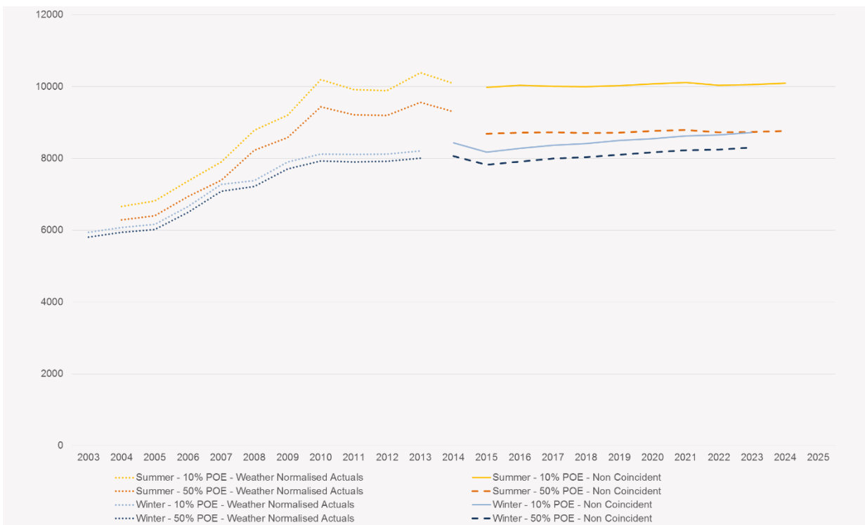
Figure 3 50% and 10% POE non-coincident aggregated connection point forecasts for Victoria
