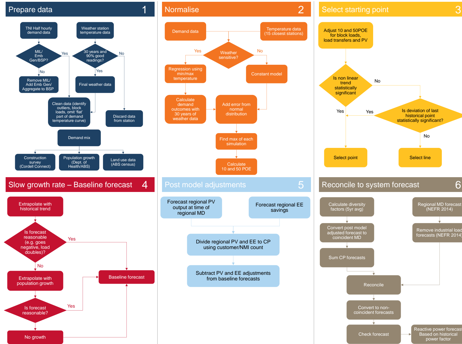
Figure 2 Implementation of forecasting methodology
