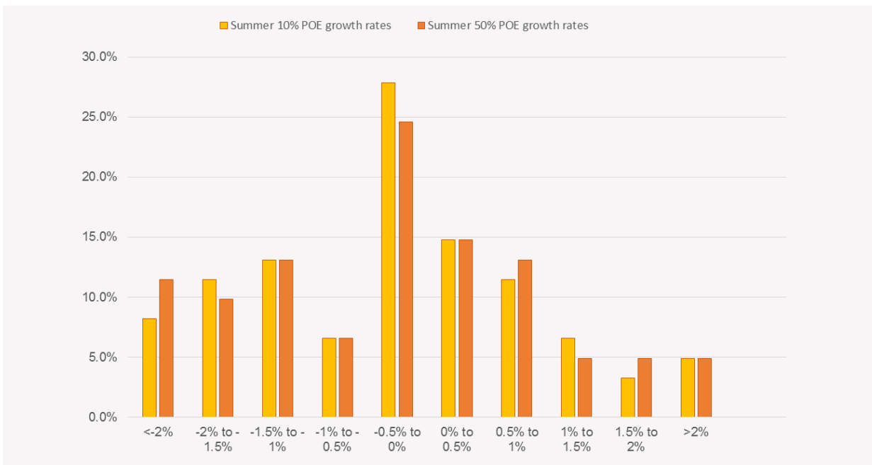
Figure 4 Distribution of summer MD growth rates for Victoria, 2015–24
