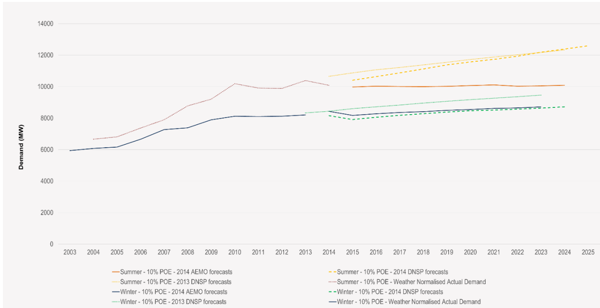
Figure 1 Aggregated 10% POE connection point forecast, compared with aggregated TSDF forecasts for 2013 and 2014.
