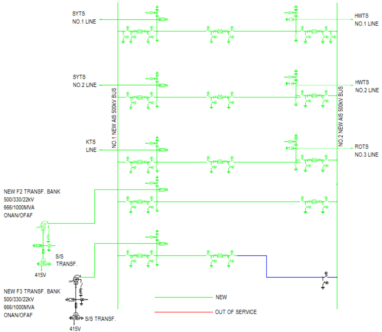
Figure 1 - SMTS 500kV SLD
