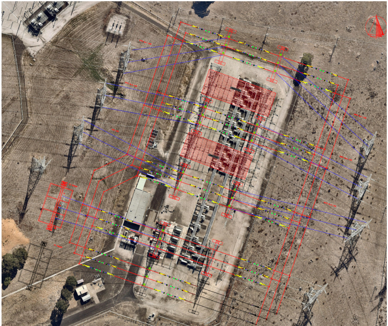
Figure 2 - SMTS 500kV SWITCHYARD POSSIBLE GENERAL ARRANGEMENT
