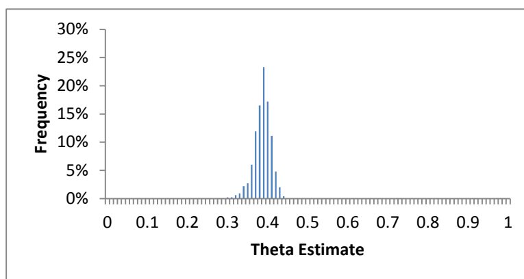
Figure 18. Histogram of theta estimates from simulation of Model 2
