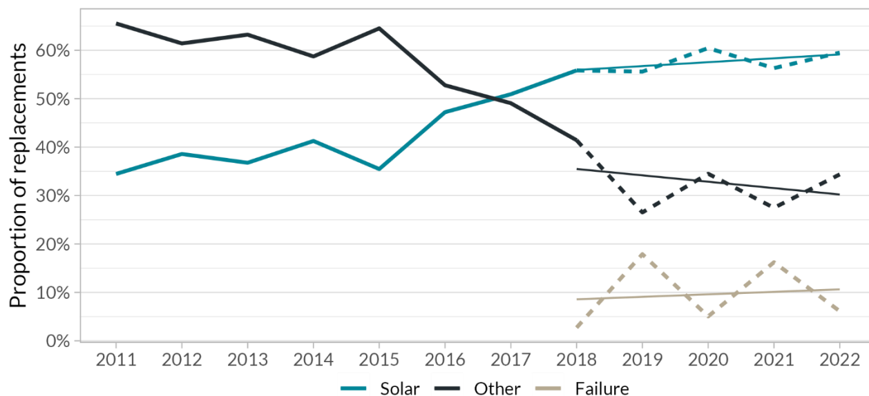
Figure 3.7: Evoenergy – replacements by driver as a proportion of replacements
