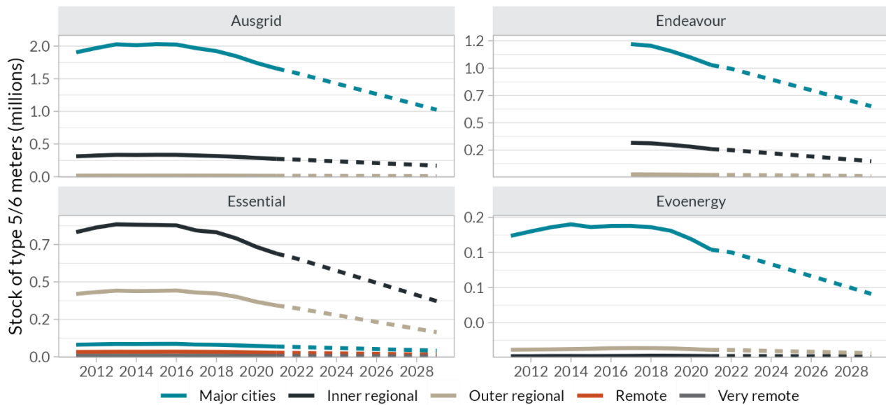
Figure 3.4: Forecast of legacy meter stock by DNSP and remoteness area
