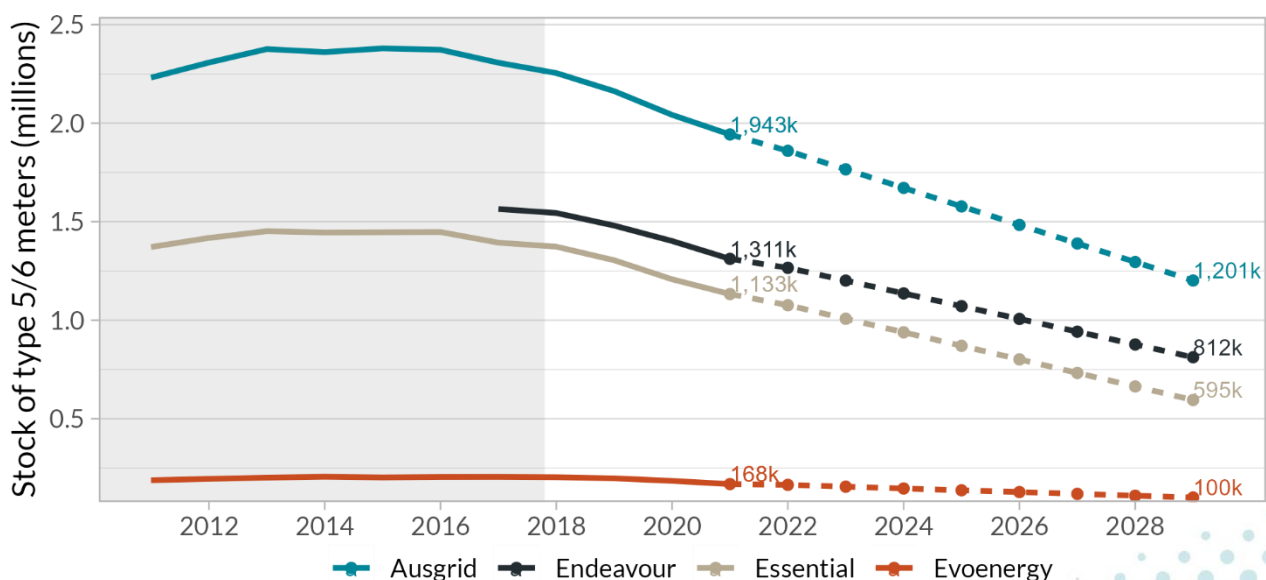
Figure 1.1: Forecast of total stock of legacy meters by DNSP
