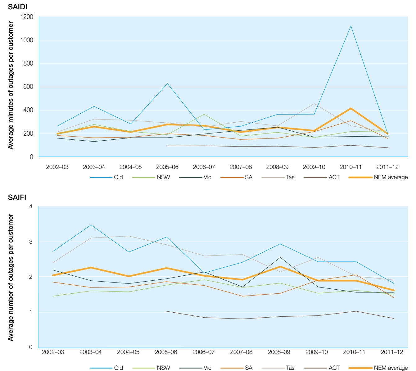
Figure 2.8 System reliability
