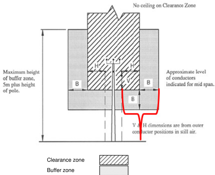
Figure 2-2: Vegetation Clearance Corridor - Non Bushfire Risk Area 132kV to 275kV
