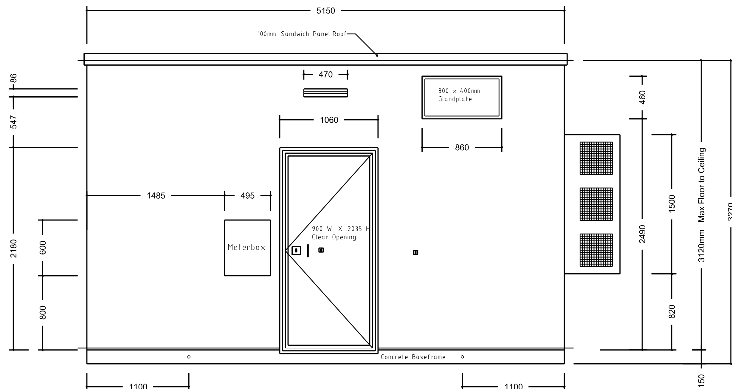
ELEVATION A SCALE: Not To Scale
