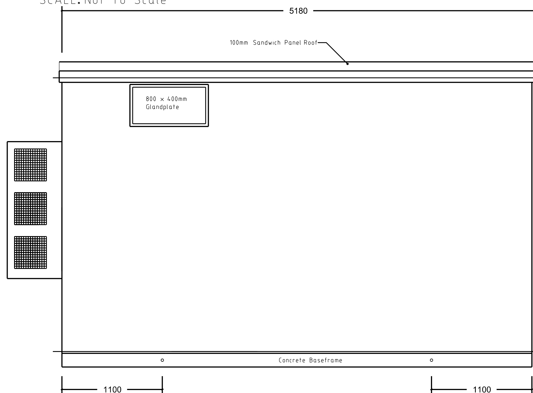
ELEVATION C SCALE: Not To Scale
