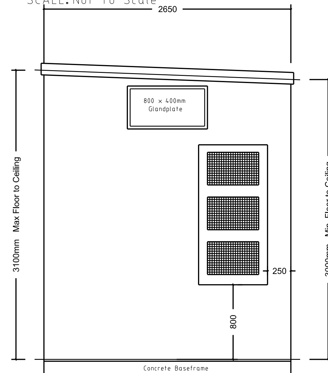
ELEVATION B SCALE: Not To Scale
