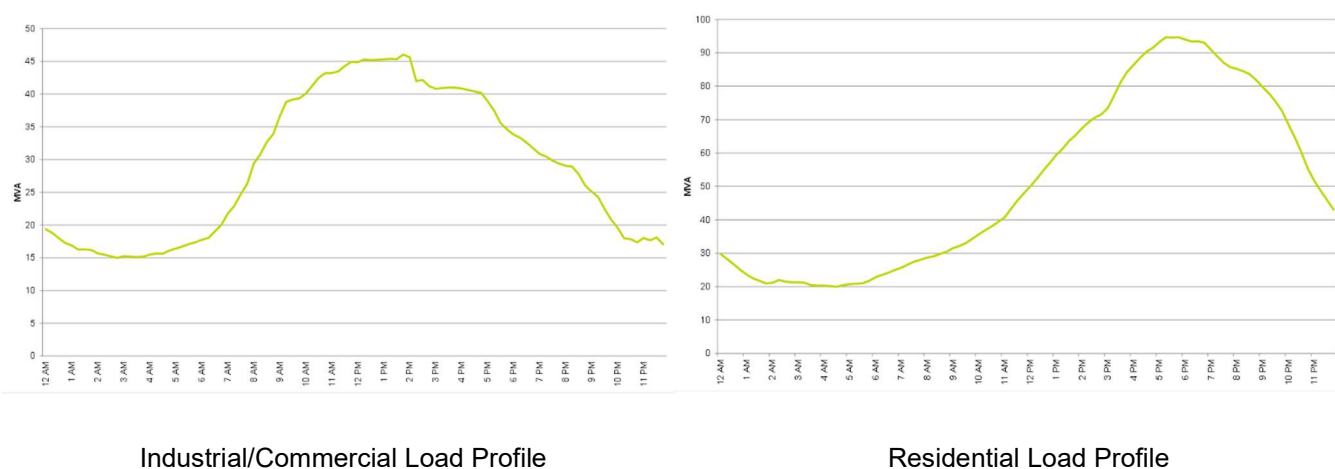
Figure 1: Typical Industrial/Commercial and Residential Load Profiles
