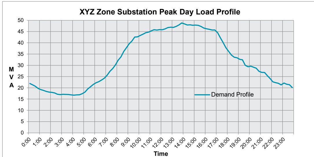
Figure B1 – XYZ Zone Substation Peak Day Profile
