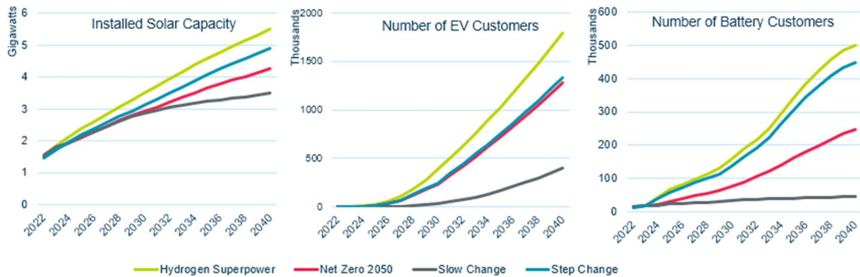
Figure 4: Projected DER uptake on the Endeavour Energy Network for the AEMO ISP Scenarios
