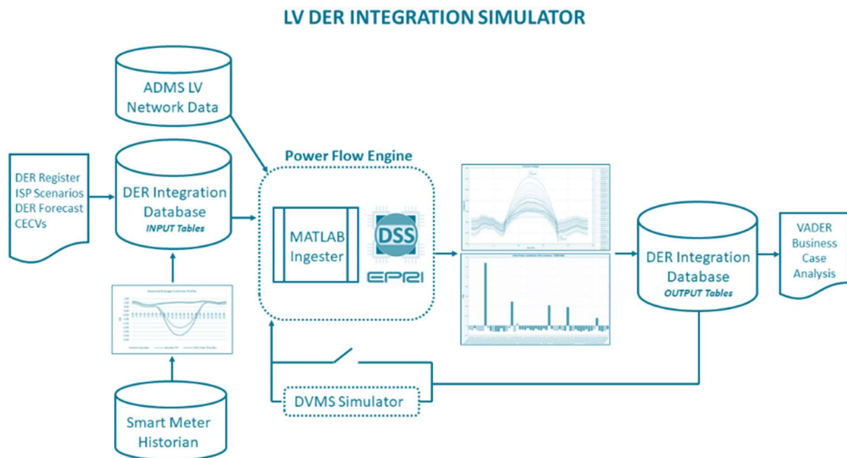
Figure 5: Explanation of inputs and flows for the DER Integration simulator
