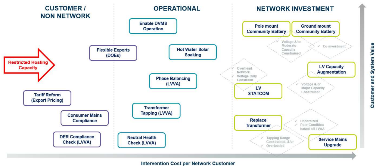
Figure 6: Classification and ranking of how hosting capacity constraints can be resolved
