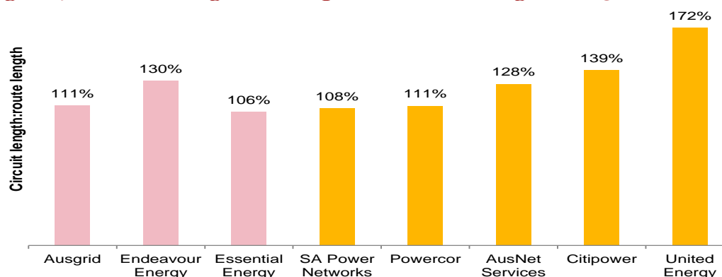
Figure 9 – Circuit length as compared to route length (2013)
