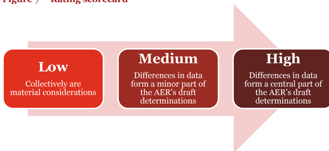
Figure 7 – Rating scorecard
