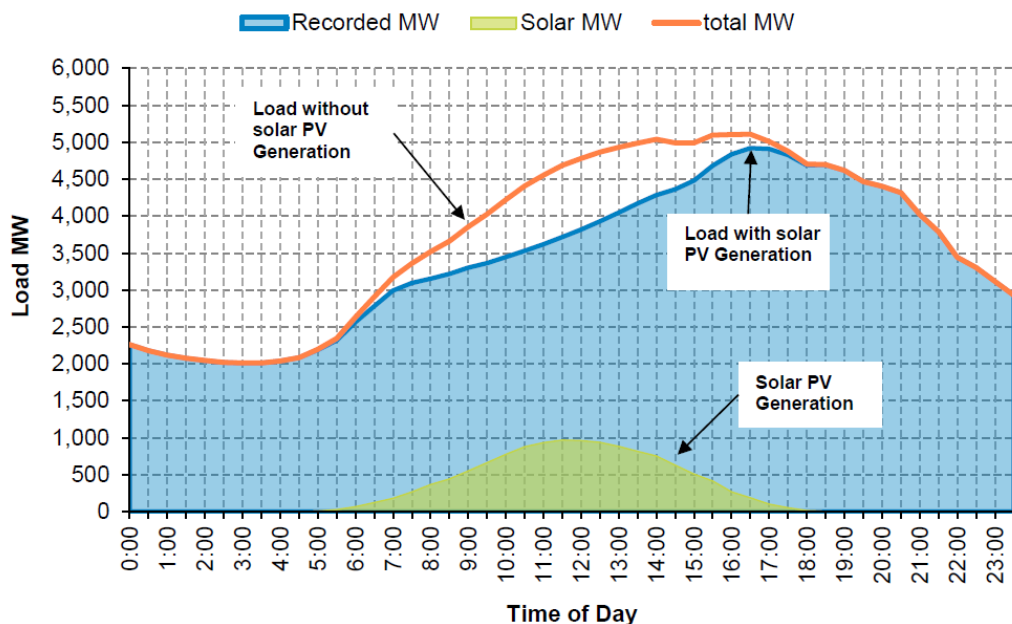
Figure 8: Energex System Demand 14 February 2018
