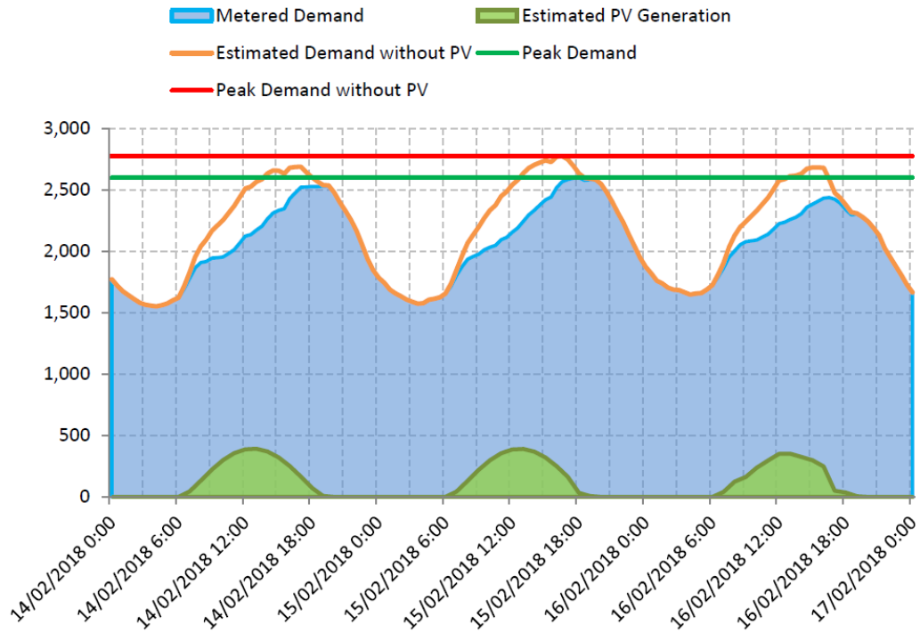
Figure 9: Ergon Energy System Demand – Solar PV Impact, 14-16 February 2018
