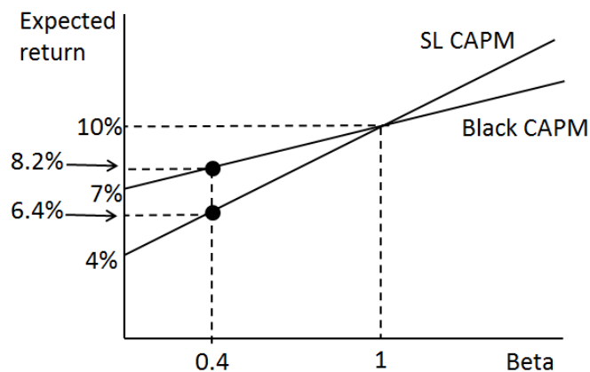
Figure 16: Comparison of SL-CAPM and Black CAPM estimates
