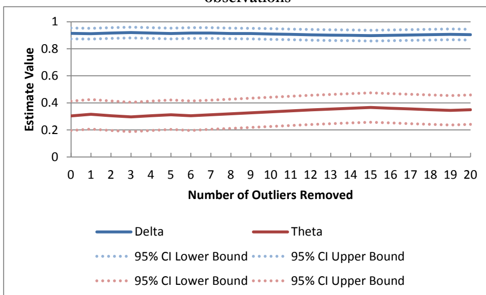
Figure 16. Sensitivity of Model 4 Delta and Theta estimates to the removal of influential observations
