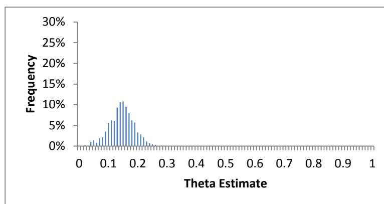
Figure 17. Histogram of theta estimates from simulation of Model 1
