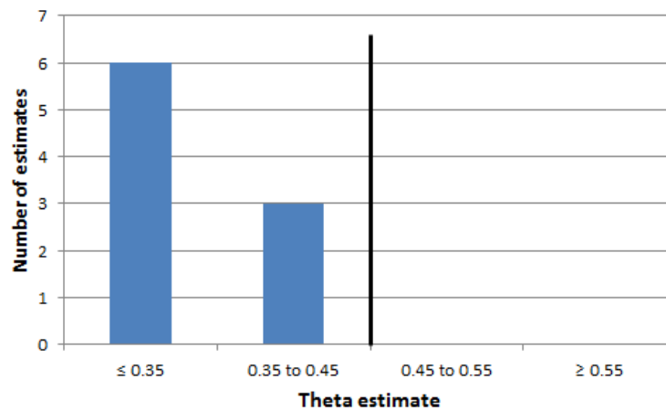
Figure 4. Distribution of ERA theta estimates: With market correction
