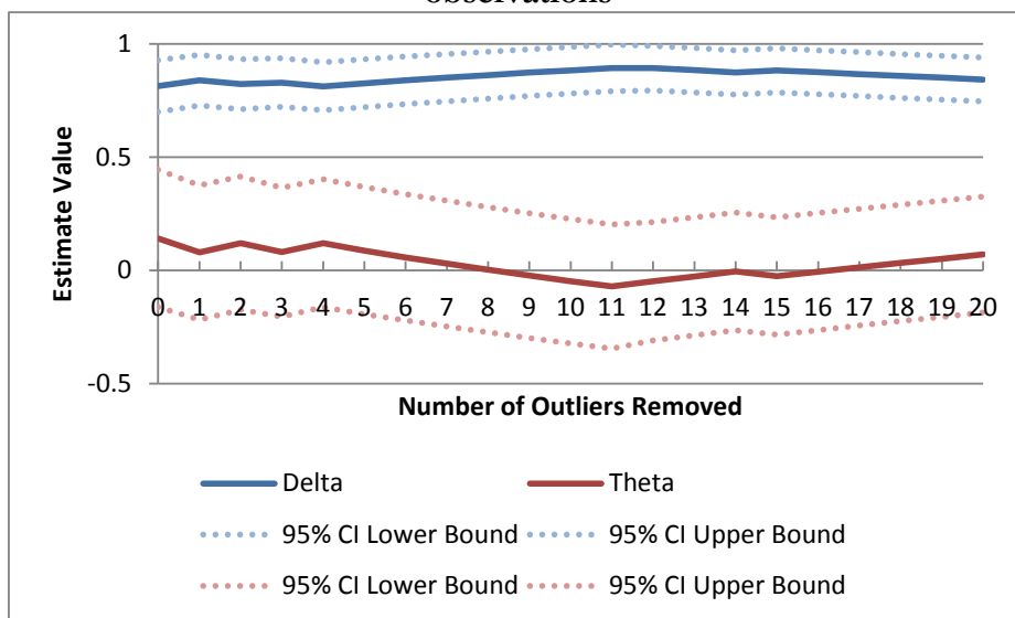
Figure 13. Sensitivity of Model 1 Delta and Theta estimates to the removal of influential observations
