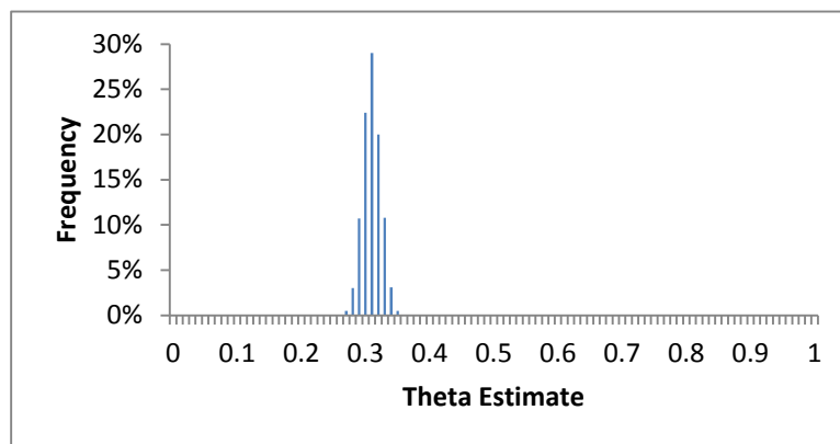
Figure 20. Histogram of theta estimates from simulation of Model 4
