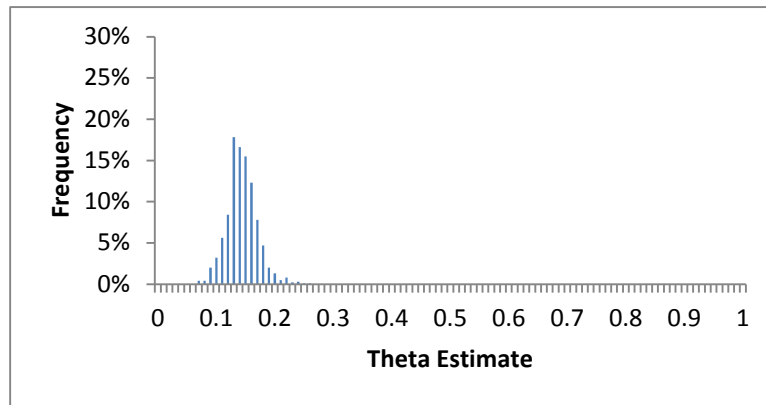
Figure 19. Histogram of theta estimates from simulation of Model 3
