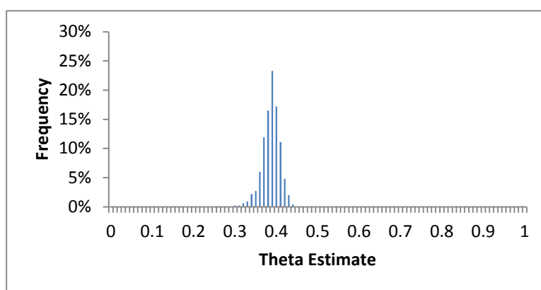
Figure 18. Histogram of theta estimates from simulation of Model 2
