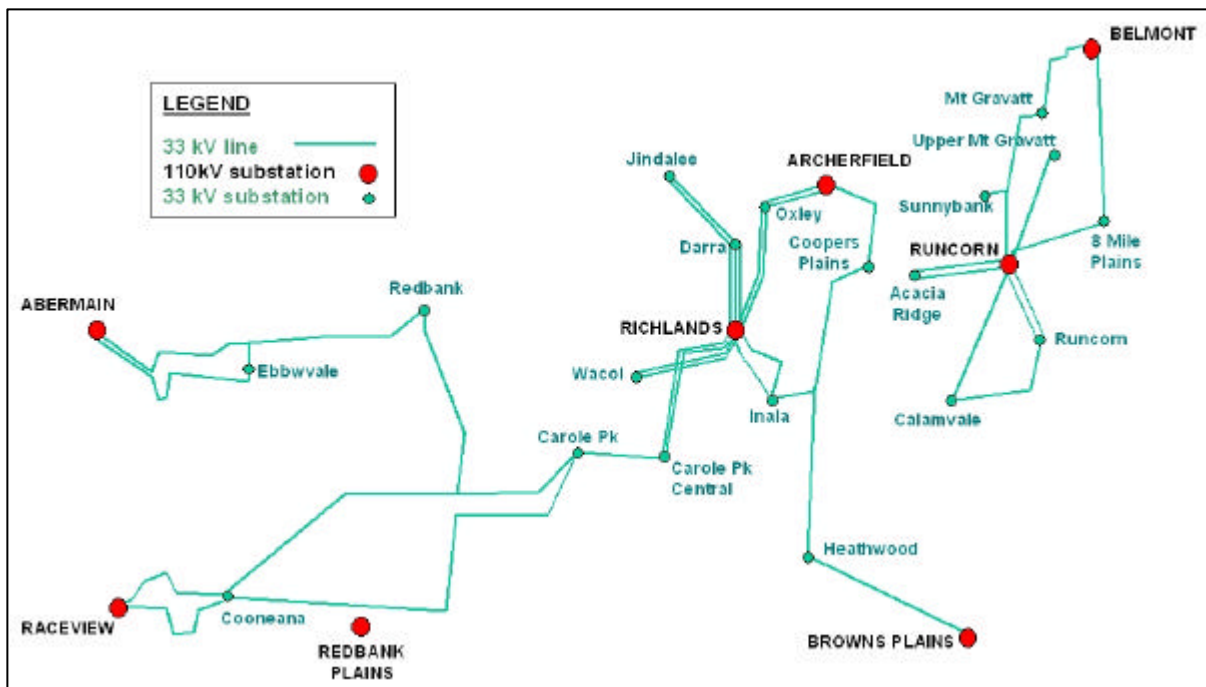
Figure 2 South West Brisbane Area Distribution Network
