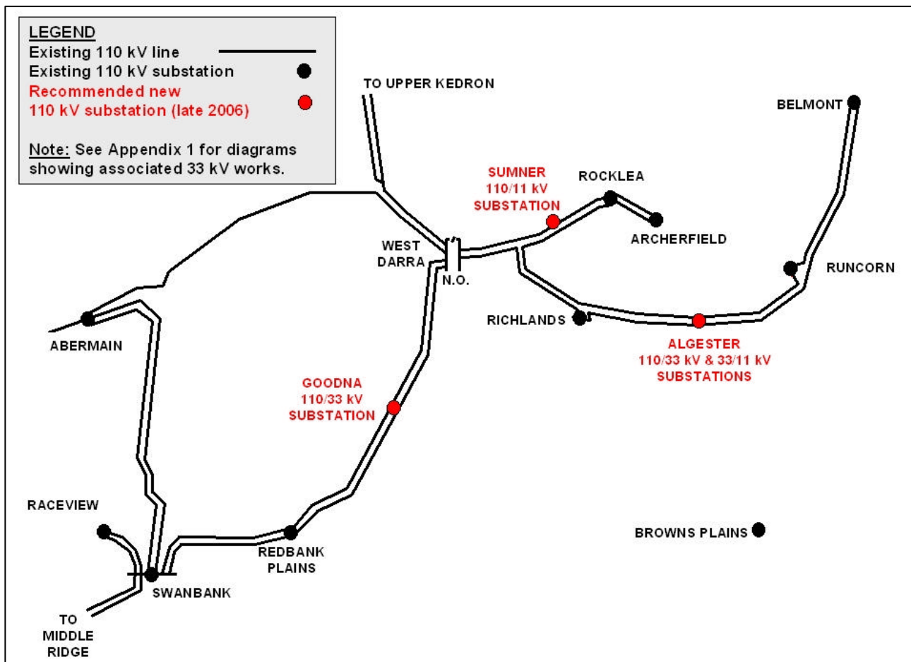
Figure 4 Option 1 – Establish New 110 kV Substations at Alger, Goodna and Sumner
