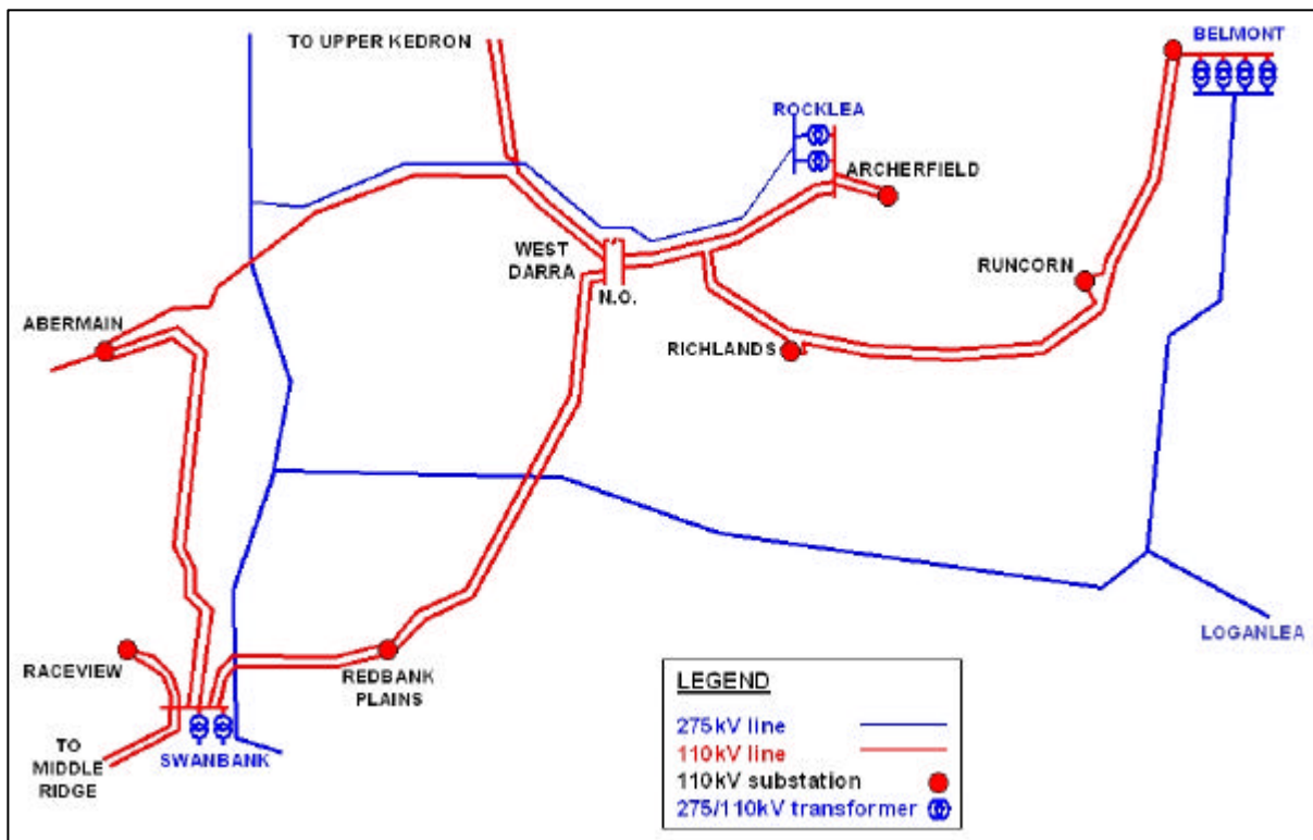
Figure 1 South West Brisbane Area Transmission Network
