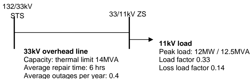
Figure 5: Existing supply arrangement
