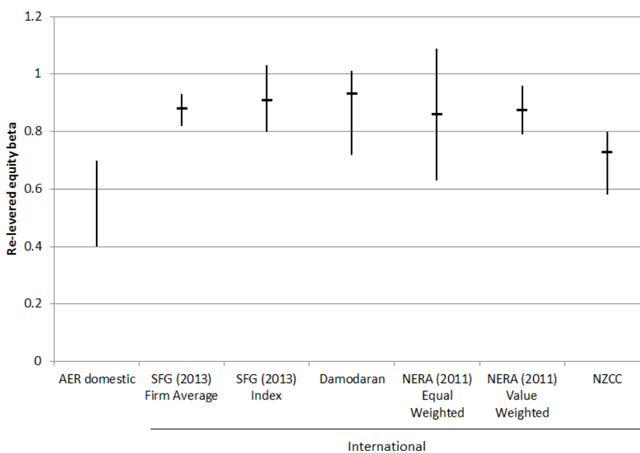
Figure 7. AER empirical estimates of beta
