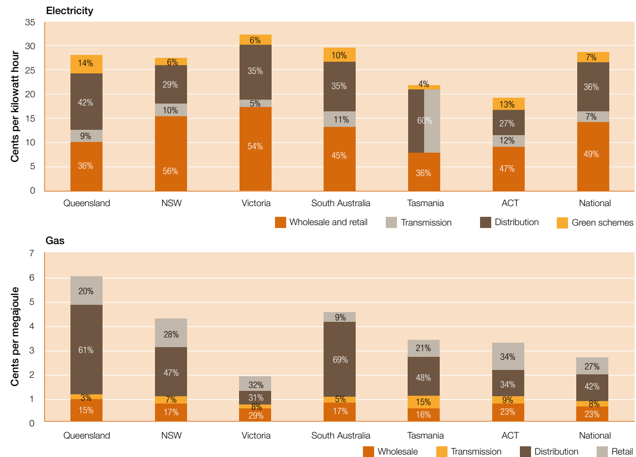
Figure 5.5 Indicative composition of residential energy bills, 2015
