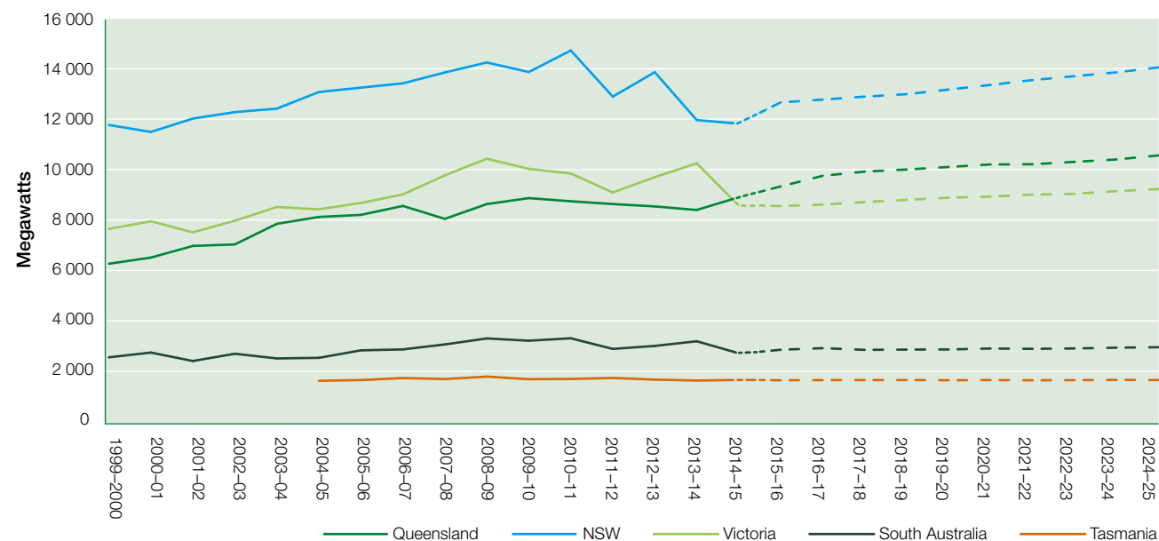
Figure 1.2 Maximum demand, and forecast maximum demand, by region
