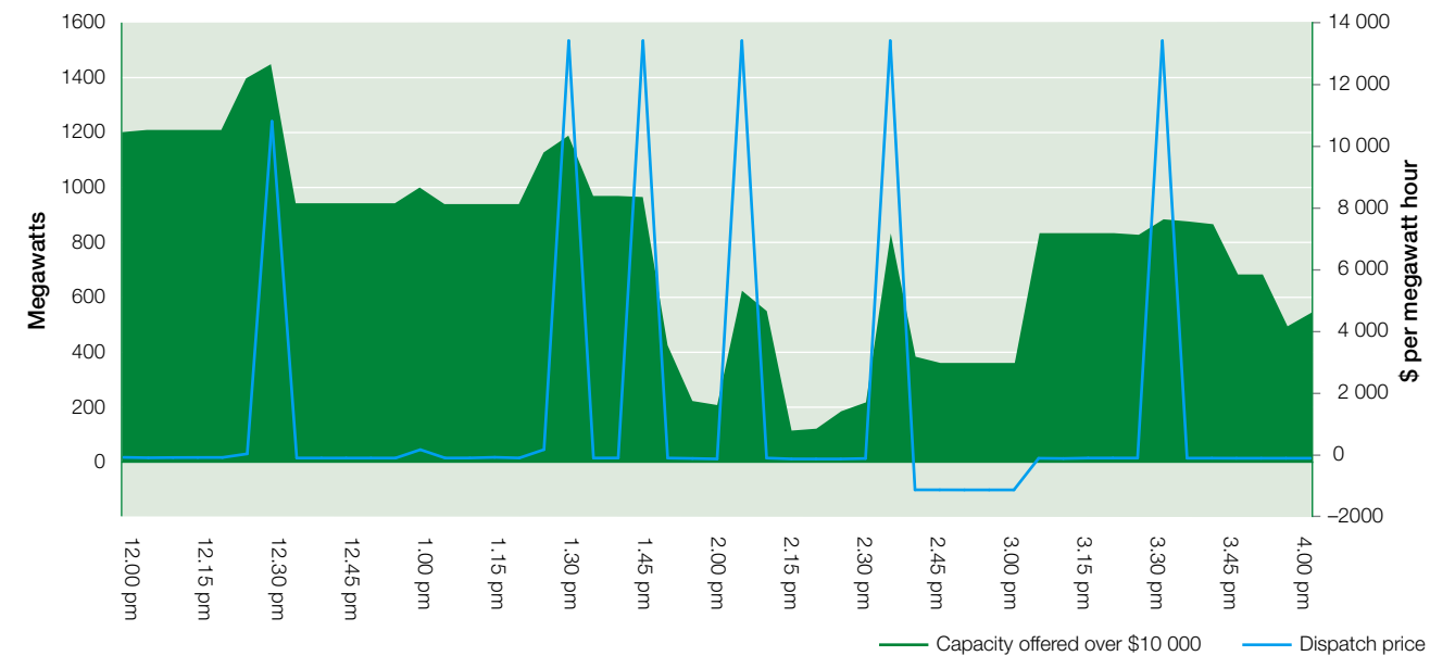
Figure 1.22 Queensland spot prices and capacity offers above $10 000 per MWh, 9 December 2014
