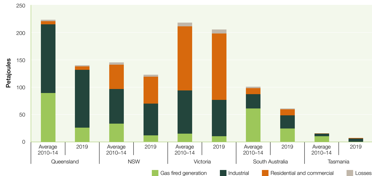
Figure 3.9 Annual domestic gas consumption, by jurisdiction
