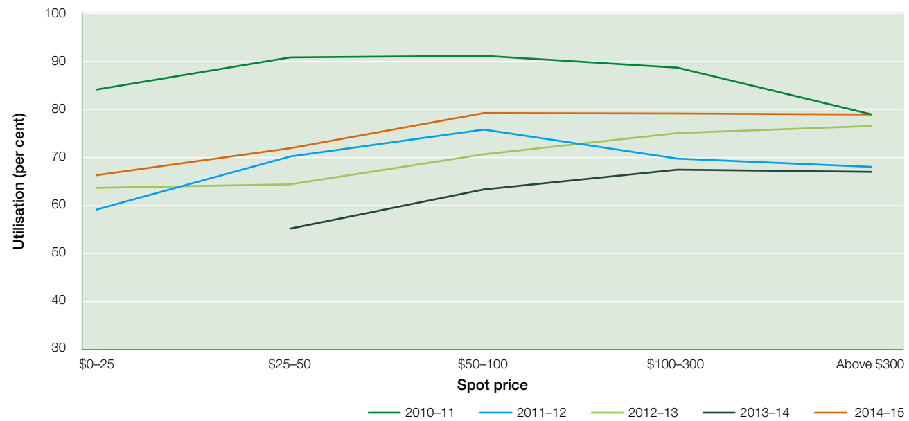
Figure 1.32 Average annual capacity use, Macquarie Generation (NSW)
