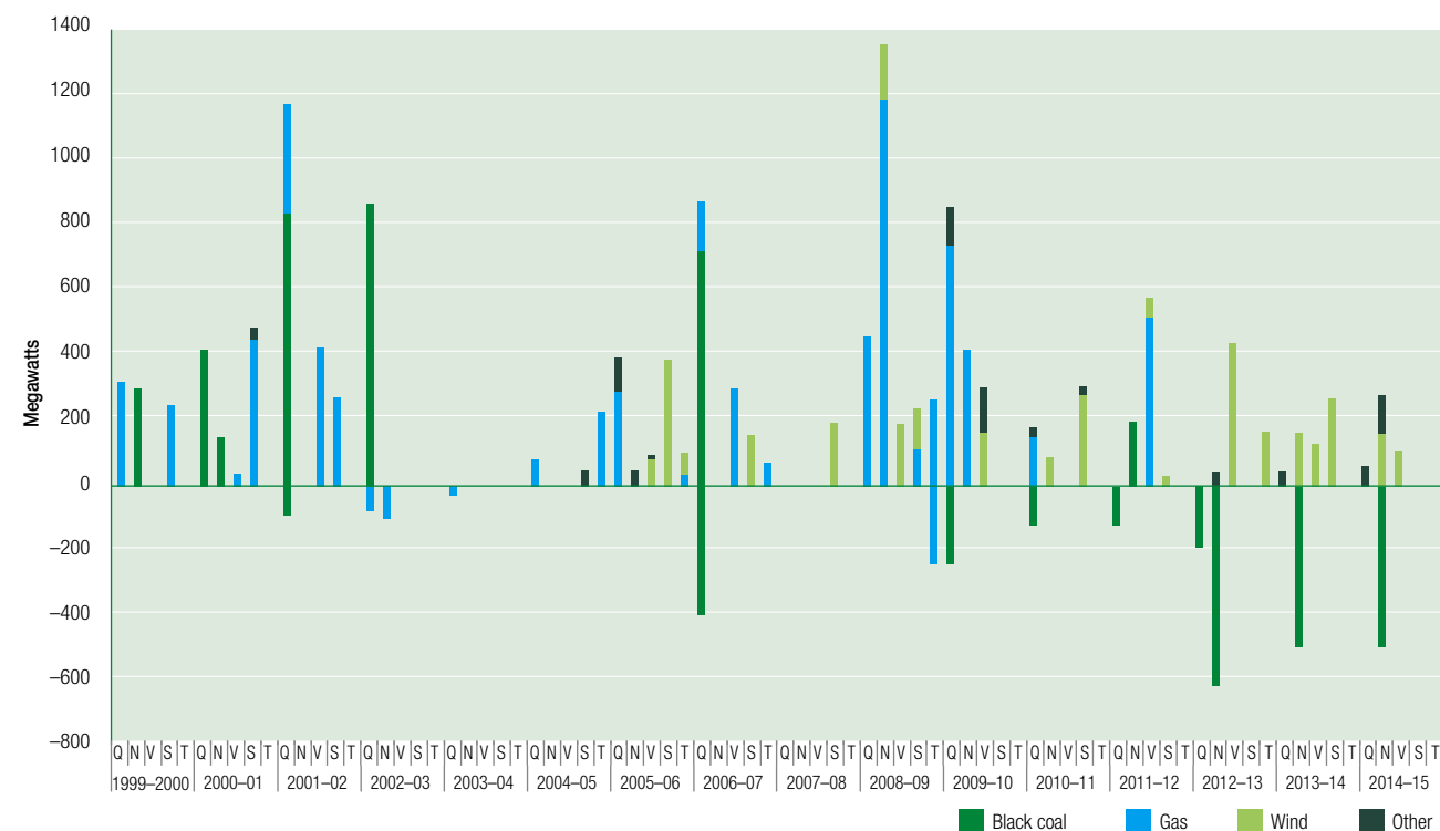
Figure 1.13 Registered generation capacity—annual investment and retirements
