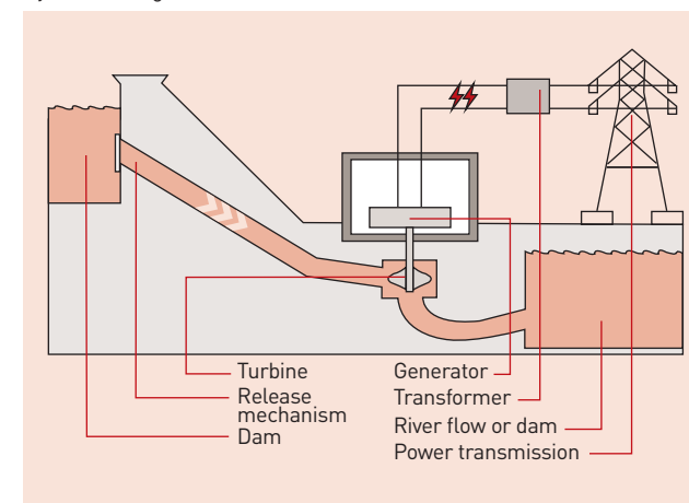
Hydroelectric generation
