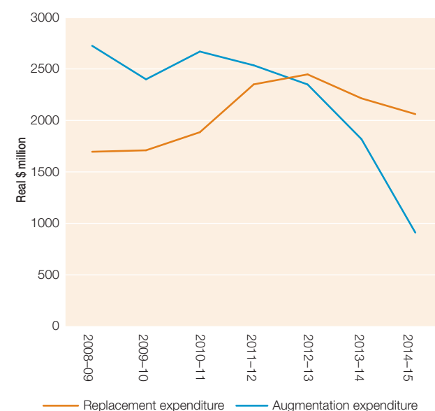
Figure 3.10 Replacement and augmentation investment—electricity networks
