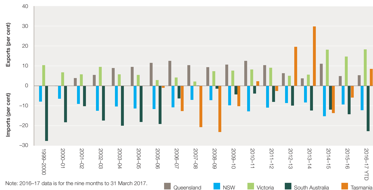
Figure 1.19 Interregional trade as a percentage of regional electricity demand
