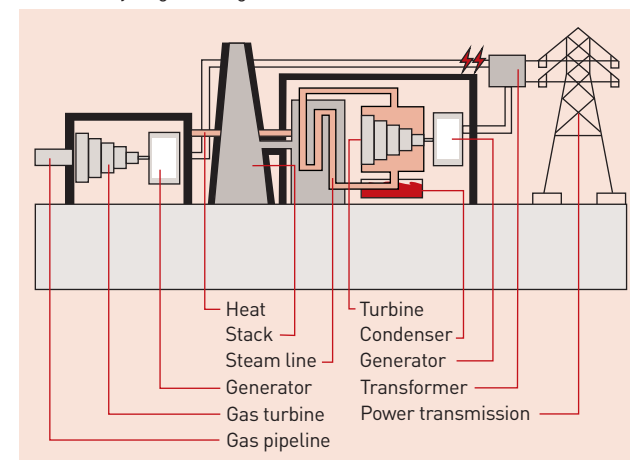
Combined cycle gas fired generation
