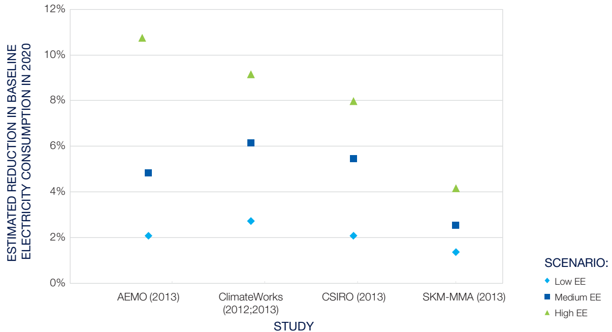
POTENTIAL IMPACTS OF ENERGY EFFICIENCY (EE) ON SYDNEY'S OVERALL ELECTRICITY CONSUMPTION IN 2020
