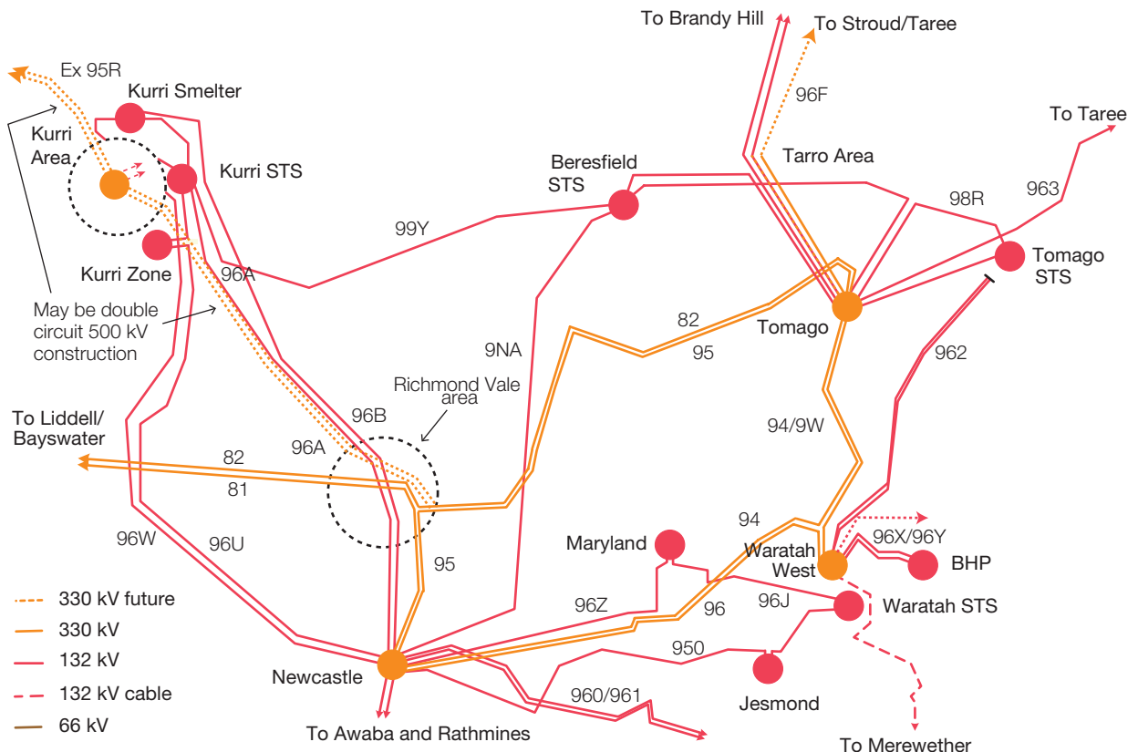
FIGURE 4.17 TRANSMISSION NETWORK IN THE GREATER NEWCASTLE AREA – INDICATIVE FUTURE
