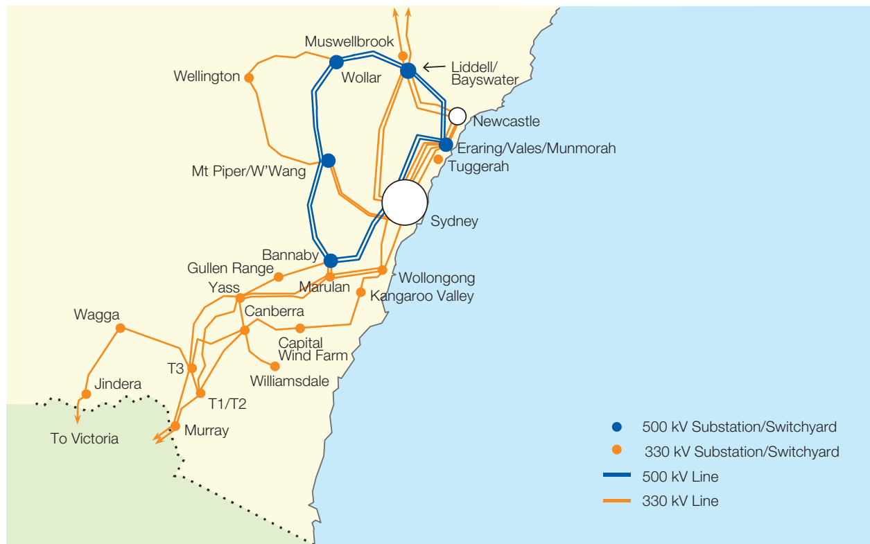
FUTURE 500 kV RING DEVELOPMENT
