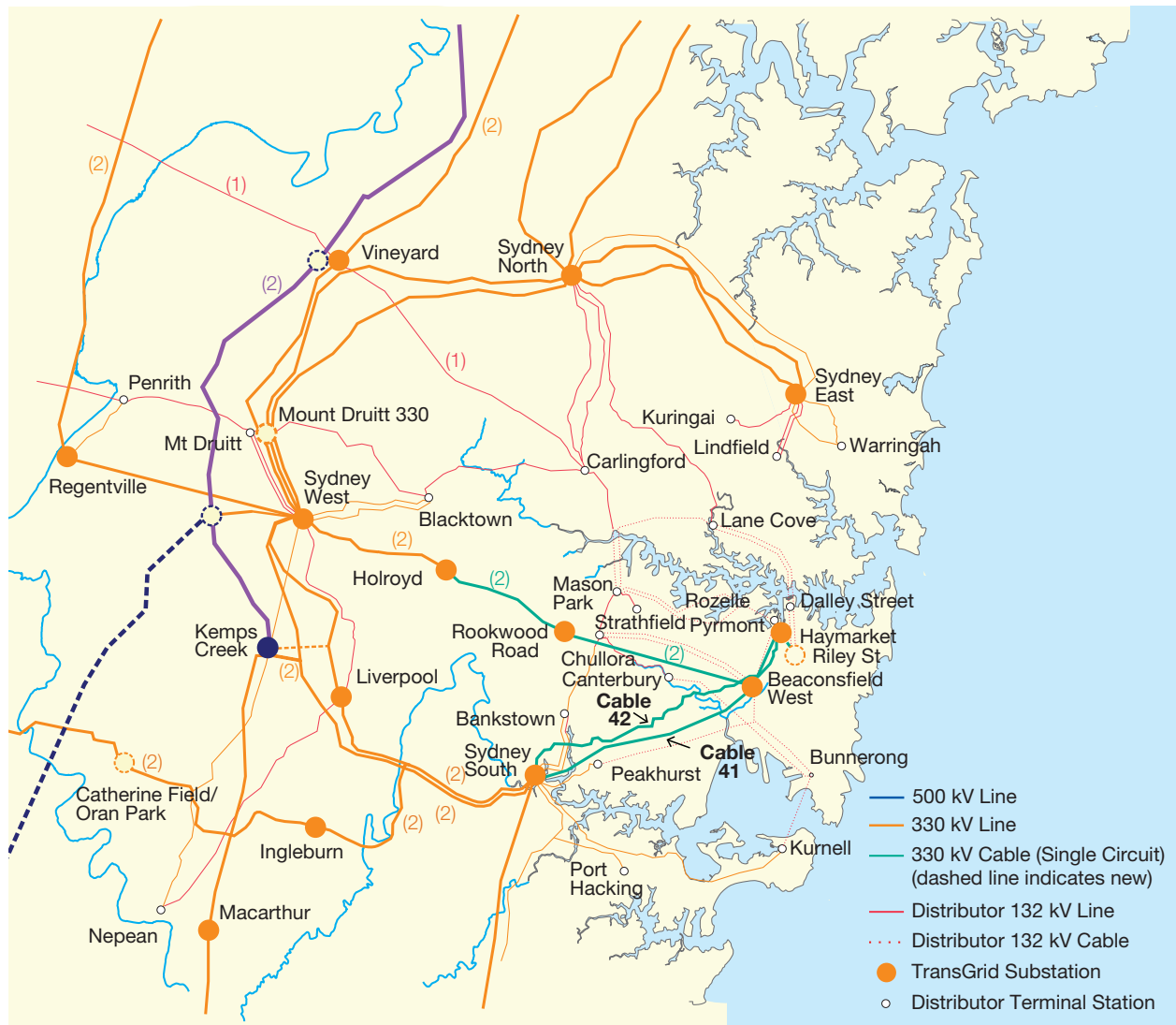
FIGURE 4.9 GREATER SYDNEY AREA NETWORK – INDICATIVE FUTURE
