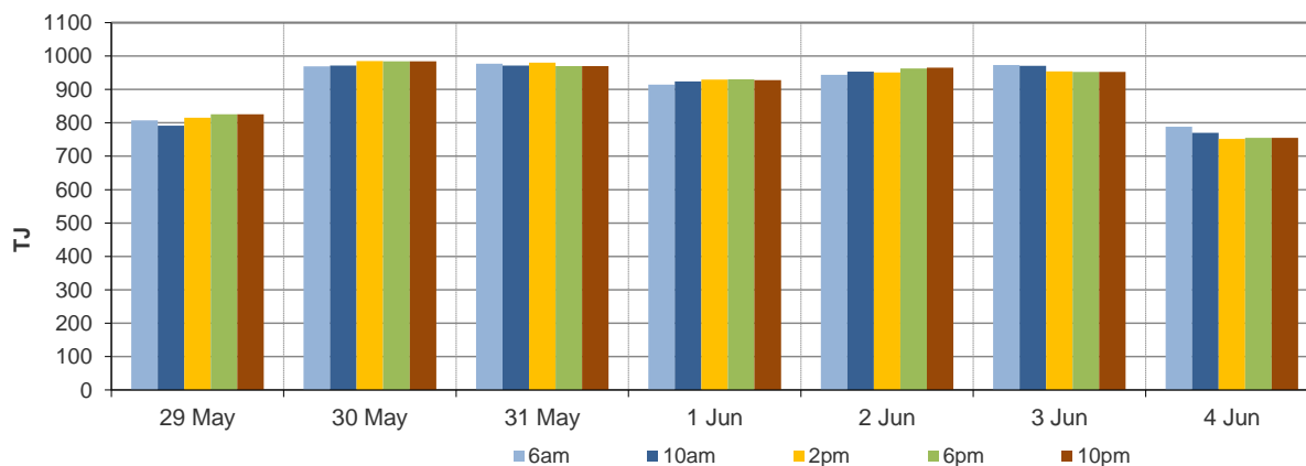
Figure 1.2: Demand forecasts
