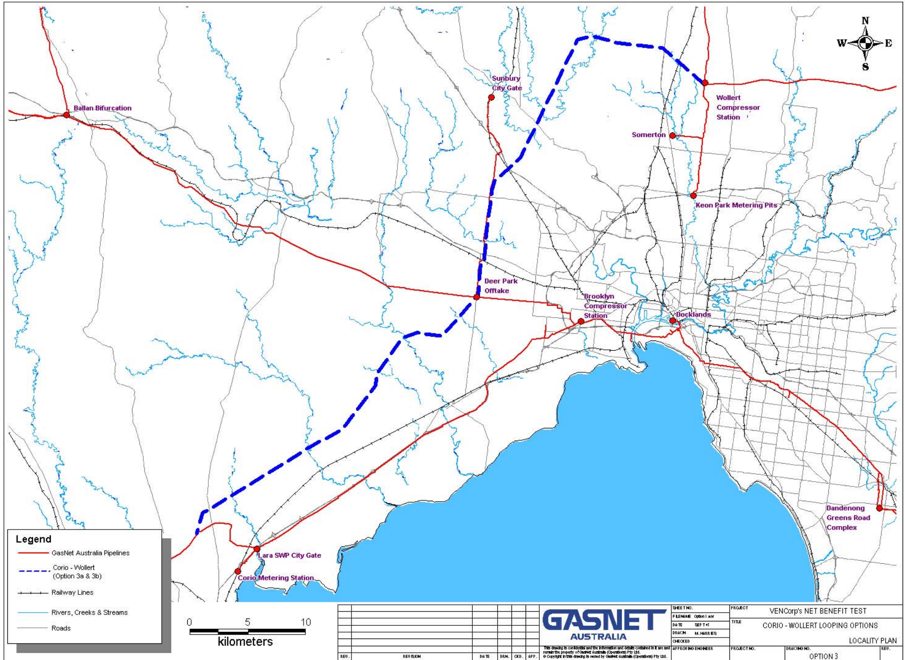
Figure 3 - Corio to Wollert augmentation
