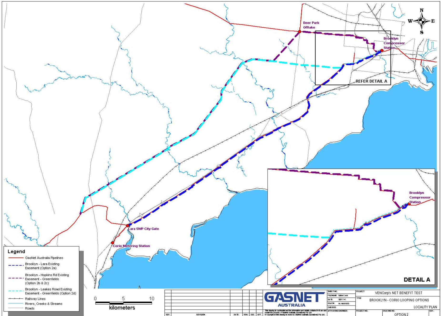
Figure 2 - Corio to Brooklyn augmentations
